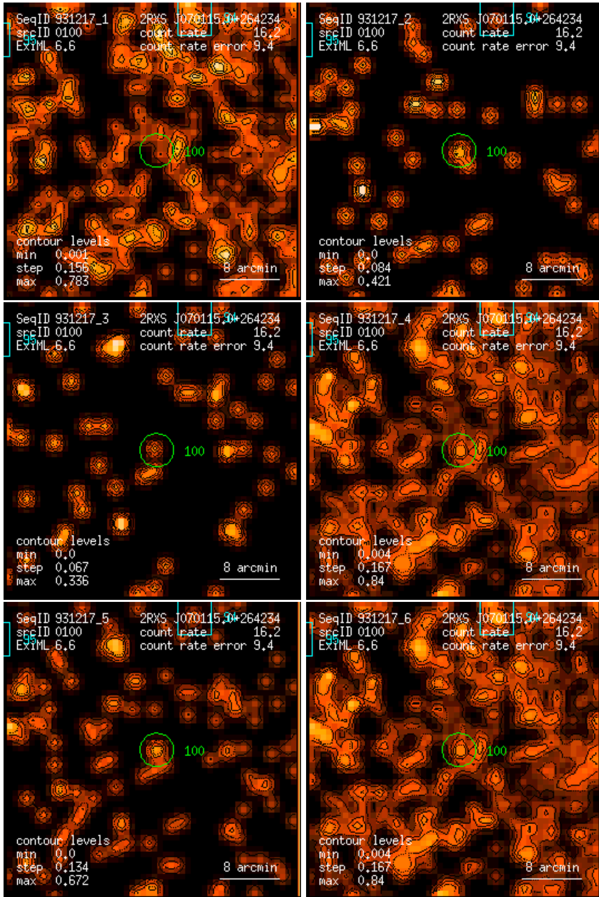
Figure 100: RASS 931217: detection 0100: band rate images, Gaussian filter: (1) PSPC channels 11 – 41, (2) 52 – 90, (3) 91 – 201, (4) 11 – 235, (5) 52 – 201, (6) 11 – 201. Broad band rates in counts/ks. Band rate contour levels in counts/ks/arcmin 2 .
