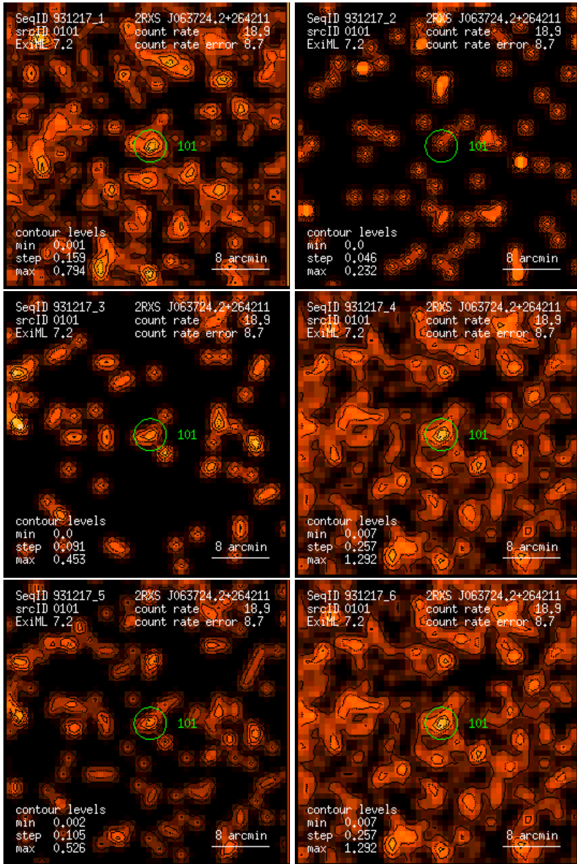
Figure 101: RASS 931217: detection 0101: band rate images, Gaussian filter: (1) PSPC channels 11 – 41, (2) 52 – 90, (3) 91 – 201, (4) 11 – 235, (5) 52 – 201, (6) 11 – 201. Broad band rates in counts/ks. Band rate contour levels in counts/ks/arcmin 2 .
