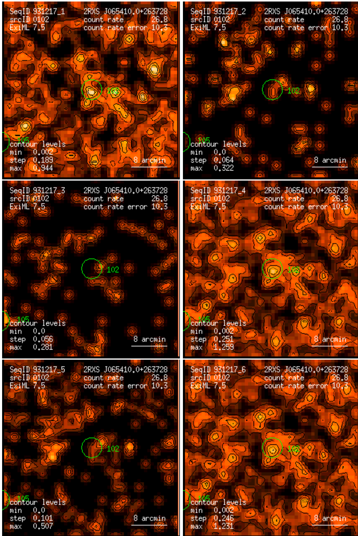
Figure 102: RASS 931217: detection 0102: band rate images, Gaussian filter: (1) PSPC channels 11 – 41, (2) 52 – 90, (3) 91 – 201, (4) 11 – 235, (5) 52 – 201, (6) 11 – 201. Broad band rates in counts/ks. Band rate contour levels in counts/ks/arcmin 2 .
