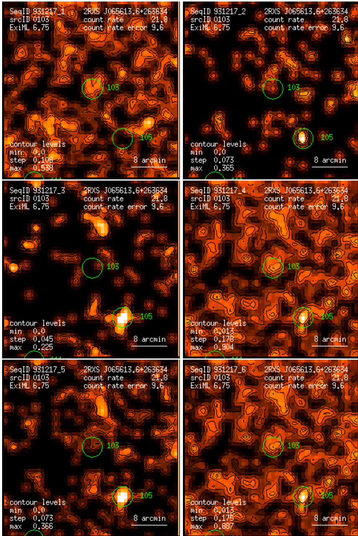
Figure 103: RASS 931217: detection 0103: band rate images, Gaussian filter: (1) PSPC channels 11 – 41, (2) 52 – 90, (3) 91 – 201, (4) 11 – 235, (5) 52 – 201, (6) 11 – 201. Broad band rates in counts/ks. Band rate contour levels in counts/ks/arcmin 2 .
