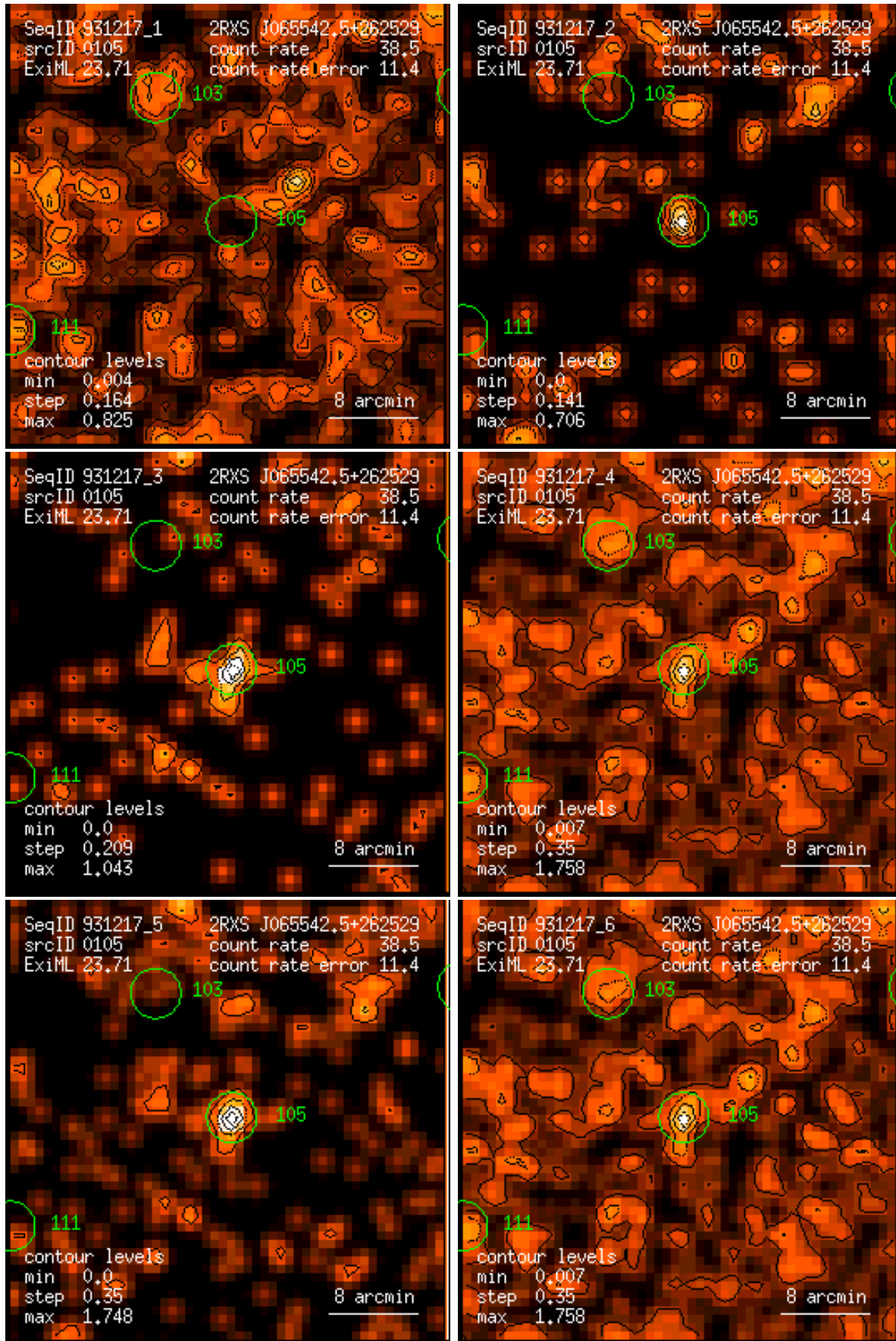
Figure 105: RASS 931217: detection 0105: band rate images, Gaussian filter: (1) PSPC channels 11 – 41, (2) 52 – 90, (3) 91 – 201, (4) 11 – 235, (5) 52 – 201, (6) 11 – 201. Broad band rates in counts/ks. Band rate contour levels in counts/ks/arcmin 2 .
