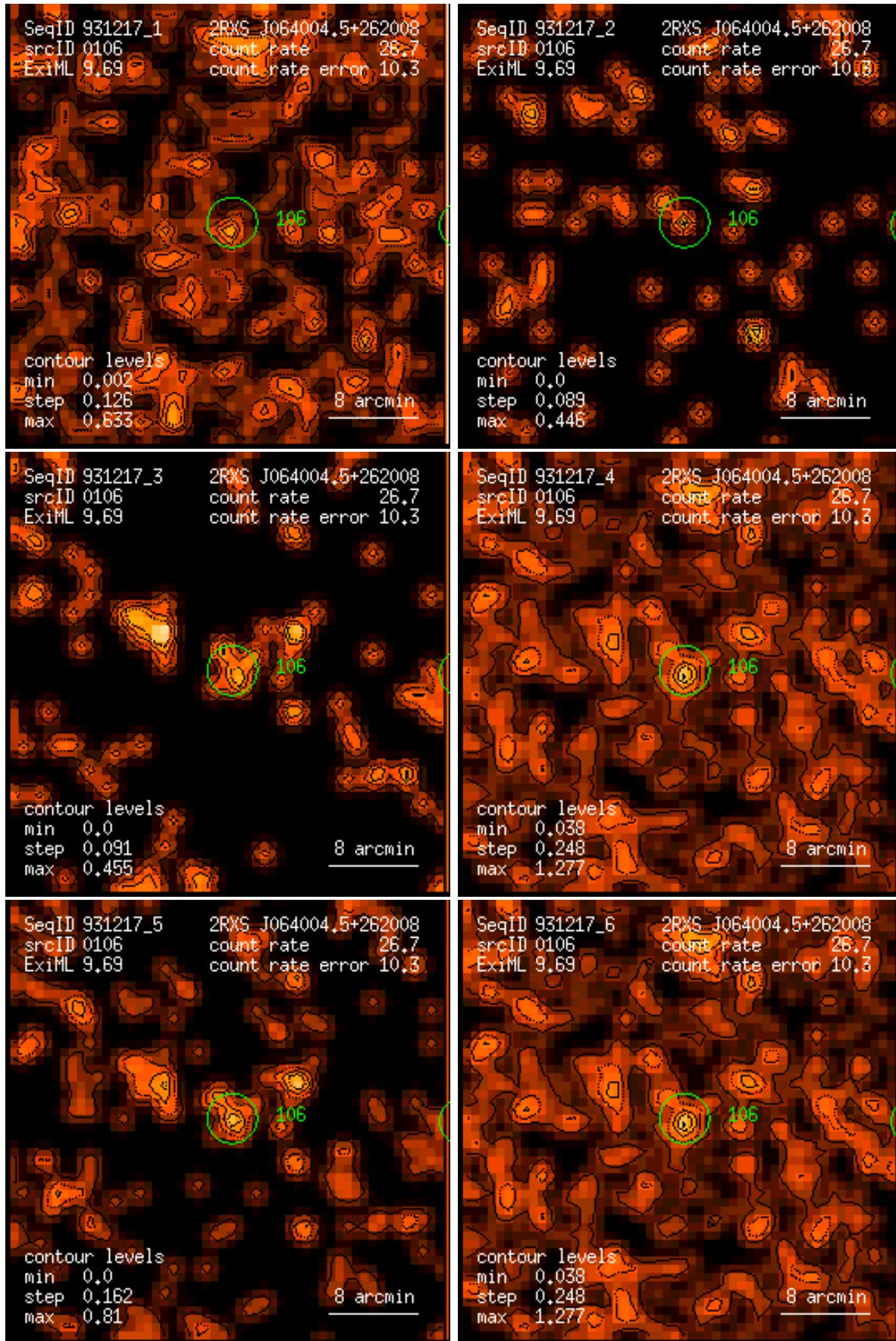
Figure 106: RASS 931217: detection 0106: band rate images, Gaussian filter: (1) PSPC channels 11 – 41, (2) 52 – 90, (3) 91 – 201, (4) 11 – 235, (5) 52 – 201, (6) 11 – 201. Broad band rates in counts/ks. Band rate contour levels in counts/ks/arcmin 2 .
