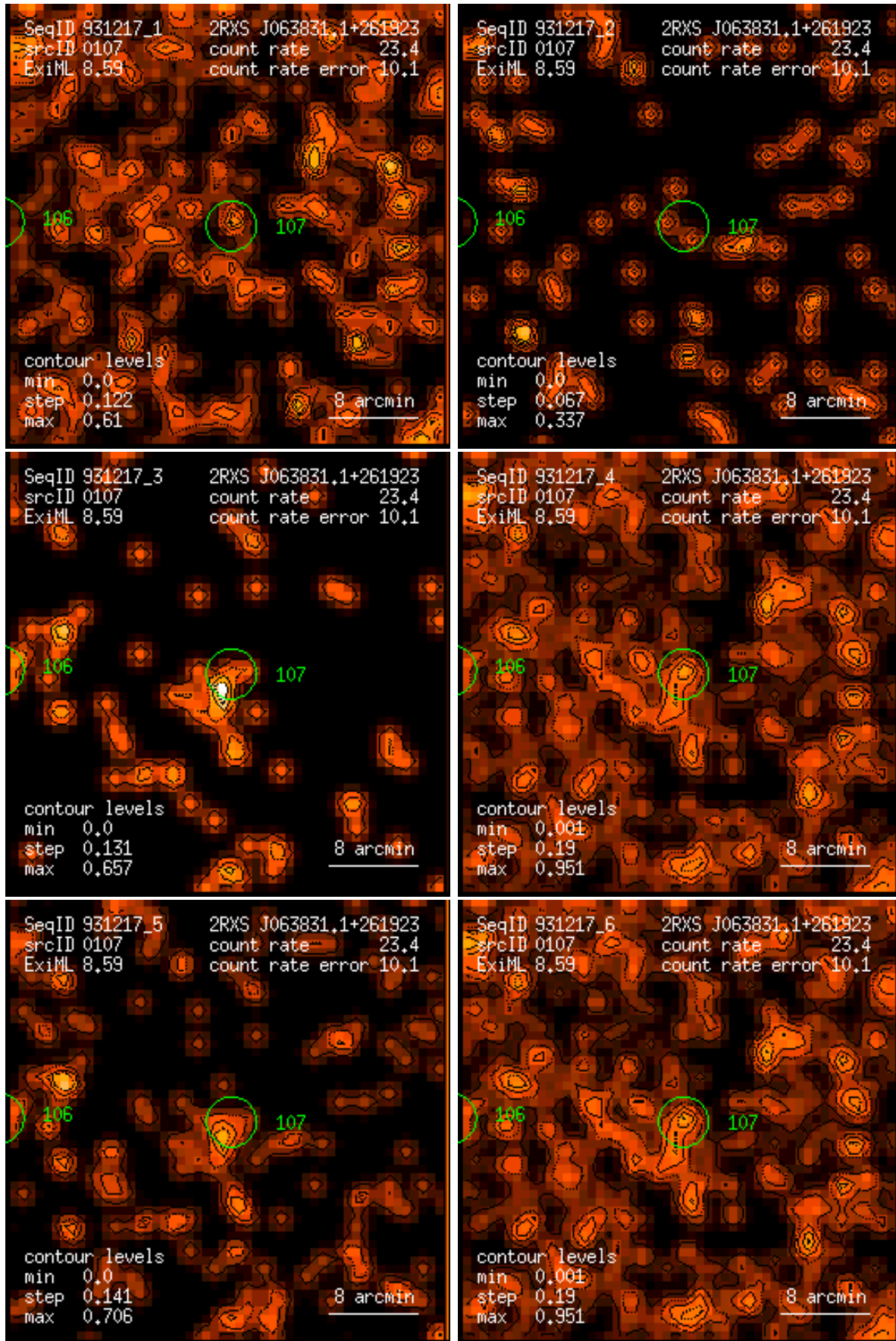
Figure 107: RASS 931217: detection 0107: band rate images, Gaussian filter: (1) PSPC channels 11 – 41, (2) 52 – 90, (3) 91 – 201, (4) 11 – 235, (5) 52 – 201, (6) 11 – 201. Broad band rates in counts/ks. Band rate contour levels in counts/ks/arcmin 2 .
