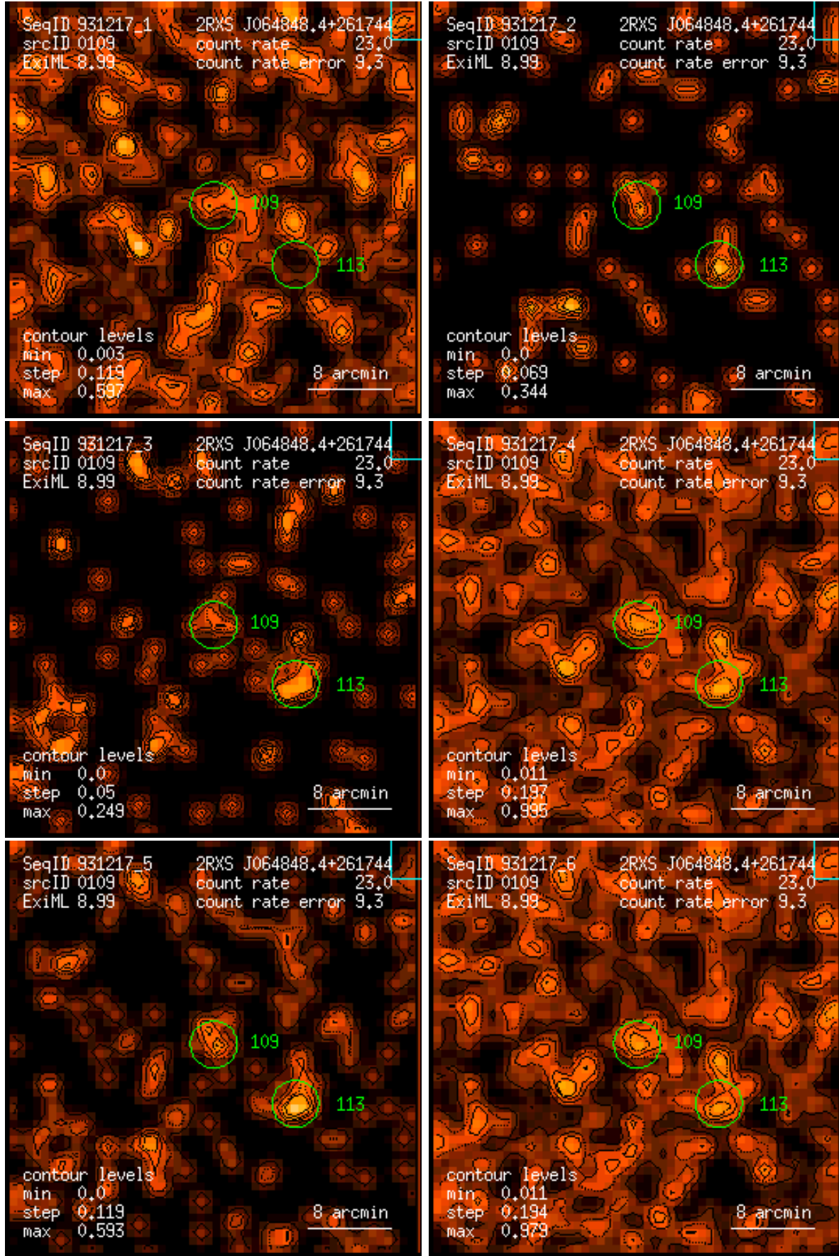
Figure 109: RASS 931217: detection 0109: band rate images, Gaussian filter: (1) PSPC channels 11 – 41, (2) 52 – 90, (3) 91 – 201, (4) 11 – 235, (5) 52 – 201, (6) 11 – 201. Broad band rates in counts/ks. Band rate contour levels in counts/ks/arcmin 2 .
