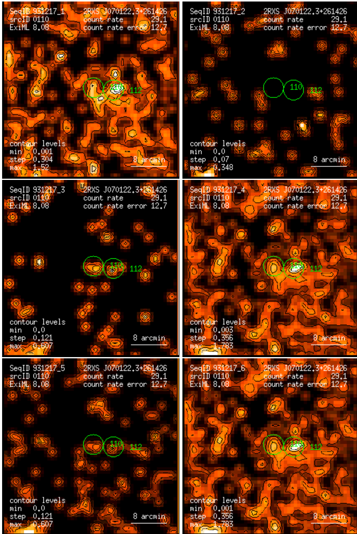
Figure 110: RASS 931217: detection 0110: band rate images, Gaussian filter: (1) PSPC channels 11 – 41, (2) 52 – 90, (3) 91 – 201, (4) 11 – 235, (5) 52 – 201, (6) 11 – 201. Broad band rates in counts/ks. Band rate contour levels in counts/ks/arcmin 2 .
