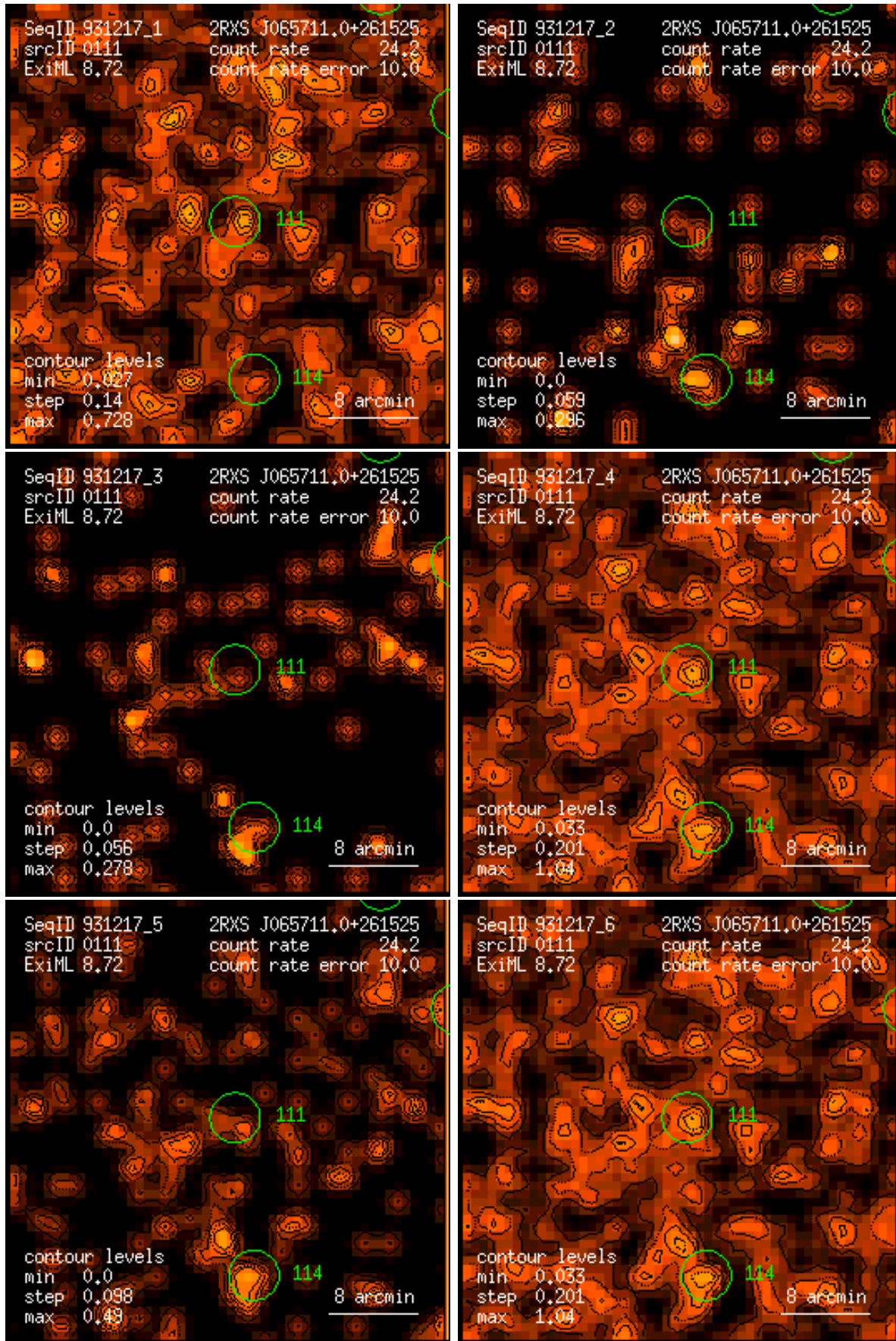
Figure 111: RASS 931217: detection 0111: band rate images, Gaussian filter: (1) PSPC channels 11 – 41, (2) 52 – 90, (3) 91 – 201, (4) 11 – 235, (5) 52 – 201, (6) 11 – 201. Broad band rates in counts/ks. Band rate contour levels in counts/ks/arcmin 2 .
