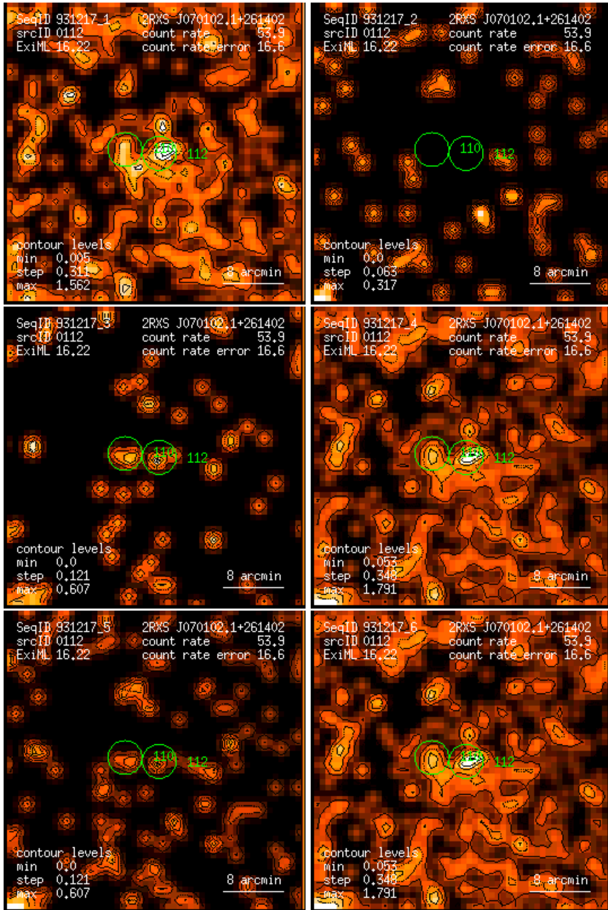
Figure 112: RASS 931217: detection 0112: band rate images, Gaussian filter: (1) PSPC channels 11 – 41, (2) 52 – 90, (3) 91 – 201, (4) 11 – 235, (5) 52 – 201, (6) 11 – 201. Broad band rates in counts/ks. Band rate contour levels in counts/ks/arcmin 2 .
