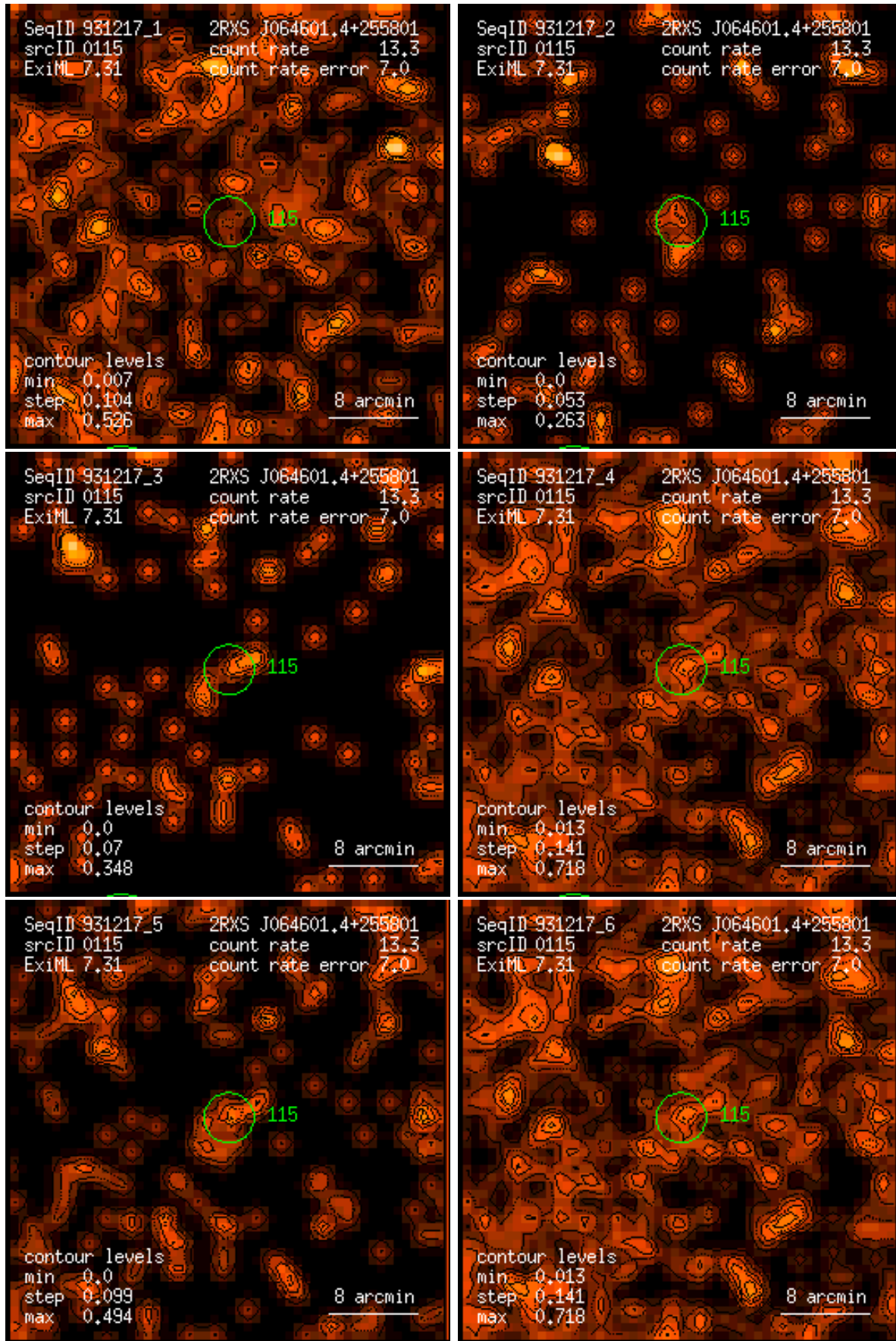
Figure 115: RASS 931217: detection 0115: band rate images, Gaussian filter: (1) PSPC channels 11 – 41, (2) 52 – 90, (3) 91 – 201, (4) 11 – 235, (5) 52 – 201, (6) 11 – 201. Broad band rates in counts/ks. Band rate contour levels in counts/ks/arcmin 2 .
