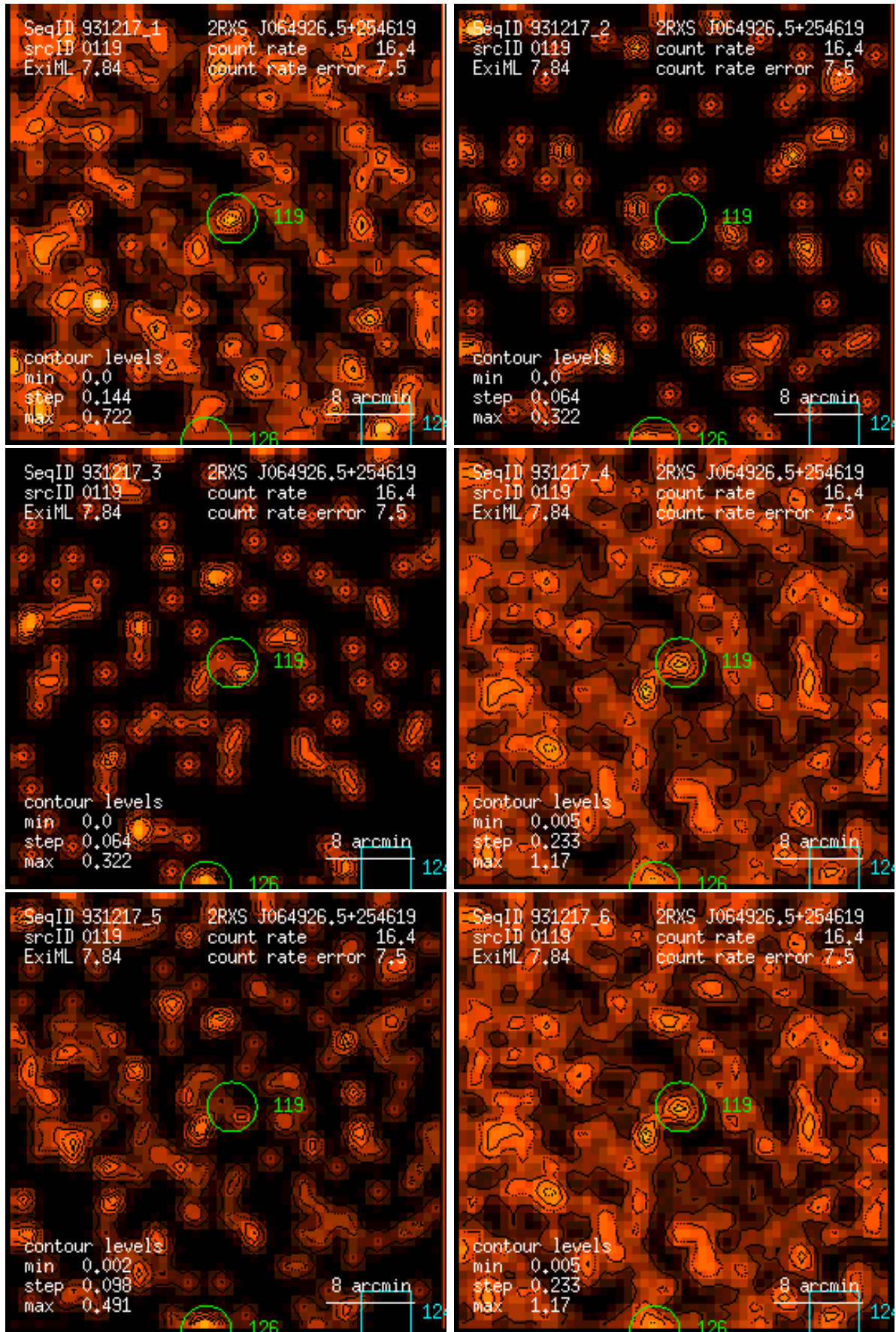
Figure 119: RASS 931217: detection 0119: band rate images, Gaussian filter: (1) PSPC channels 11 – 41, (2) 52 – 90, (3) 91 – 201, (4) 11 – 235, (5) 52 – 201, (6) 11 – 201. Broad band rates in counts/ks. Band rate contour levels in counts/ks/arcmin 2 .
