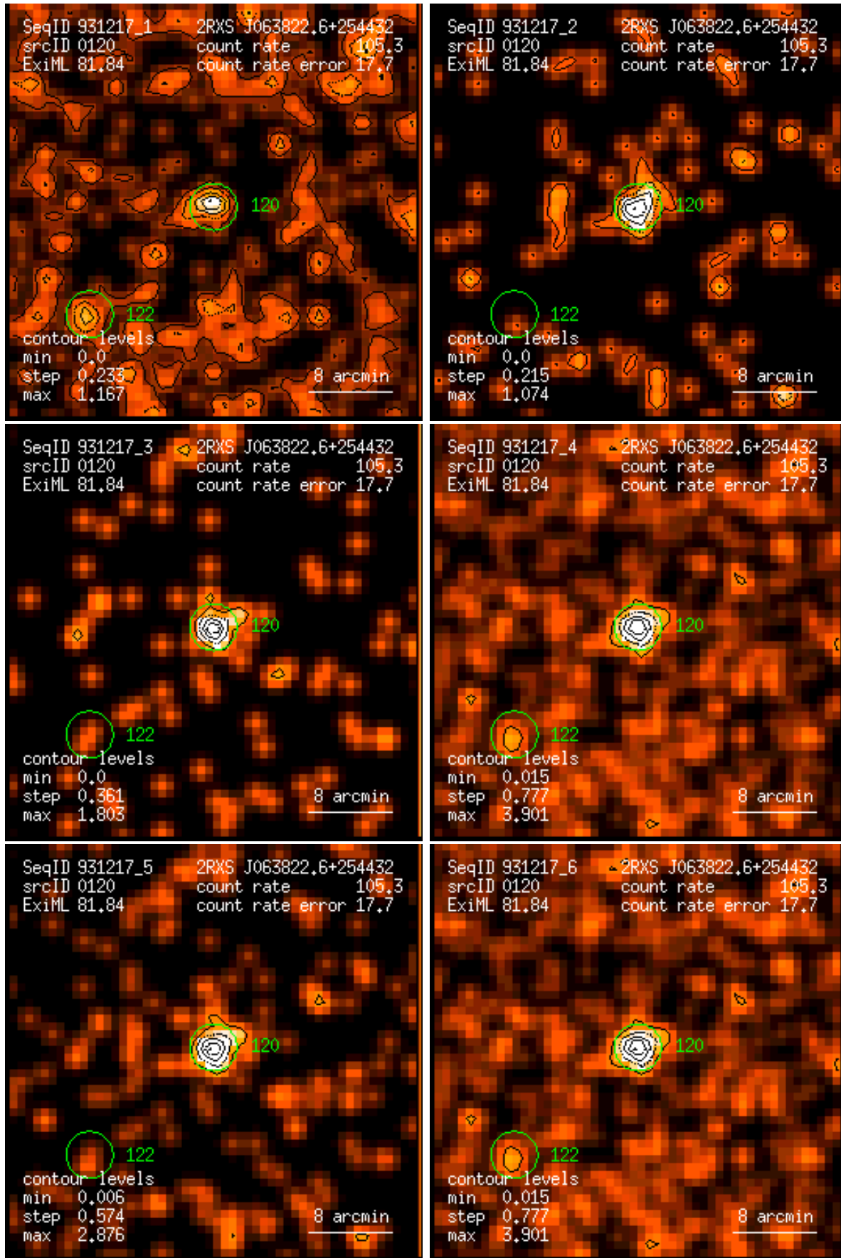
Figure 120: RASS 931217: detection 0120: band rate images, Gaussian filter: (1) PSPC channels 11 – 41, (2) 52 – 90, (3) 91 – 201, (4) 11 – 235, (5) 52 – 201, (6) 11 – 201. Broad band rates in counts/ks. Band rate contour levels in counts/ks/arcmin 2 .
