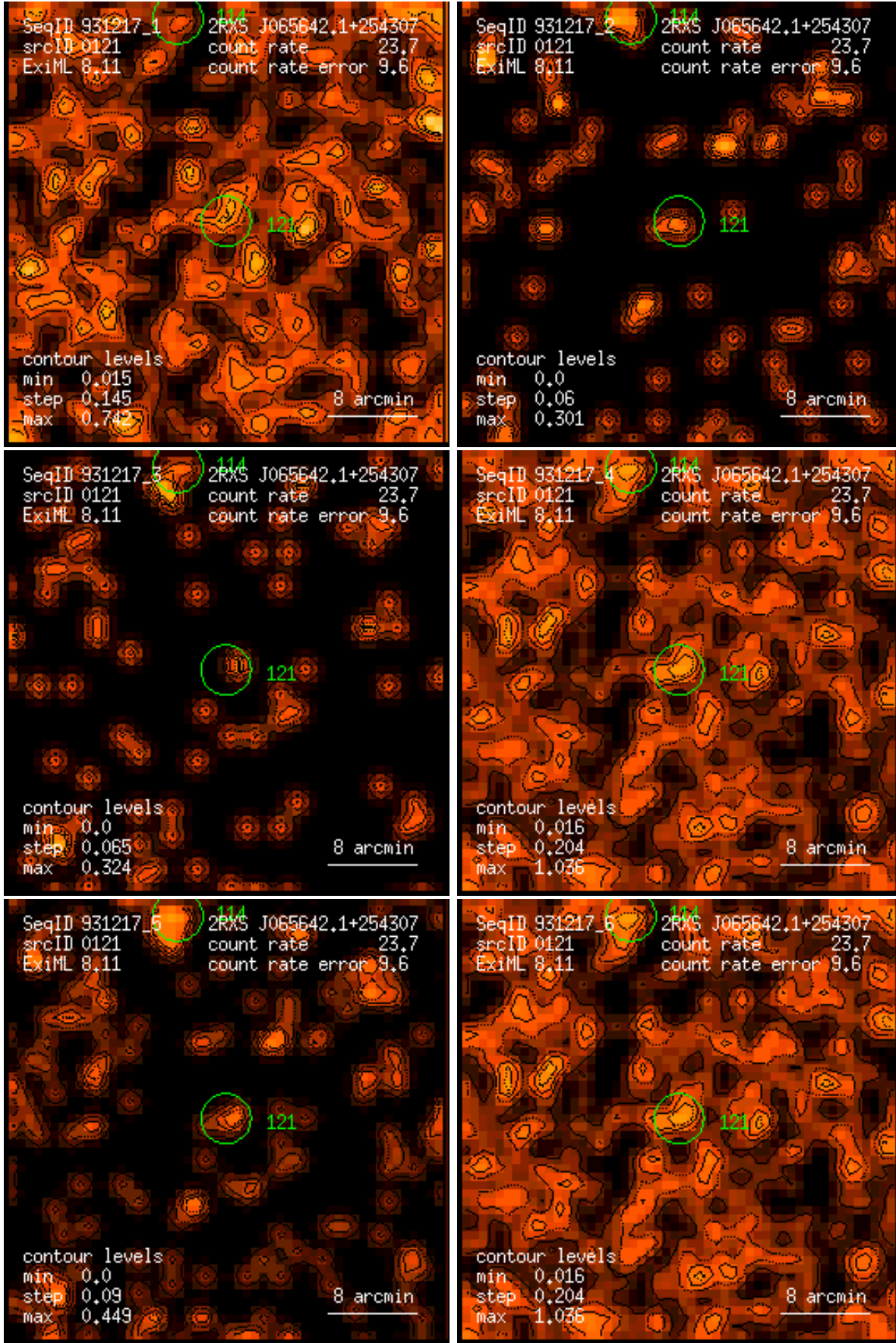
Figure 121: RASS 931217: detection 0121: band rate images, Gaussian filter: (1) PSPC channels 11 – 41, (2) 52 – 90, (3) 91 – 201, (4) 11 – 235, (5) 52 – 201, (6) 11 – 201. Broad band rates in counts/ks. Band rate contour levels in counts/ks/arcmin 2 .
