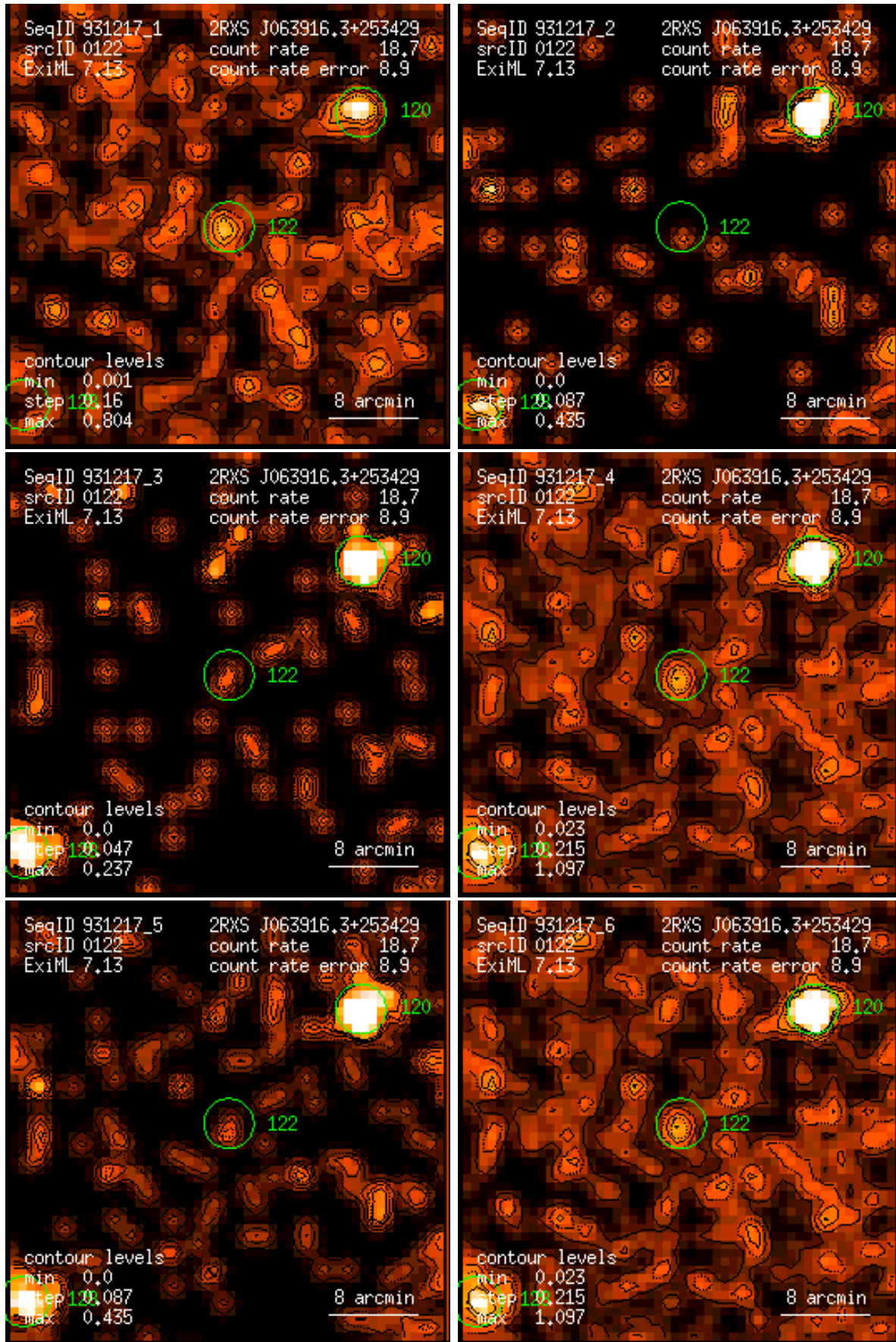
Figure 122: RASS 931217: detection 0122: band rate images, Gaussian filter: (1) PSPC channels 11 – 41, (2) 52 – 90, (3) 91 – 201, (4) 11 – 235, (5) 52 – 201, (6) 11 – 201. Broad band rates in counts/ks. Band rate contour levels in counts/ks/arcmin 2 .
