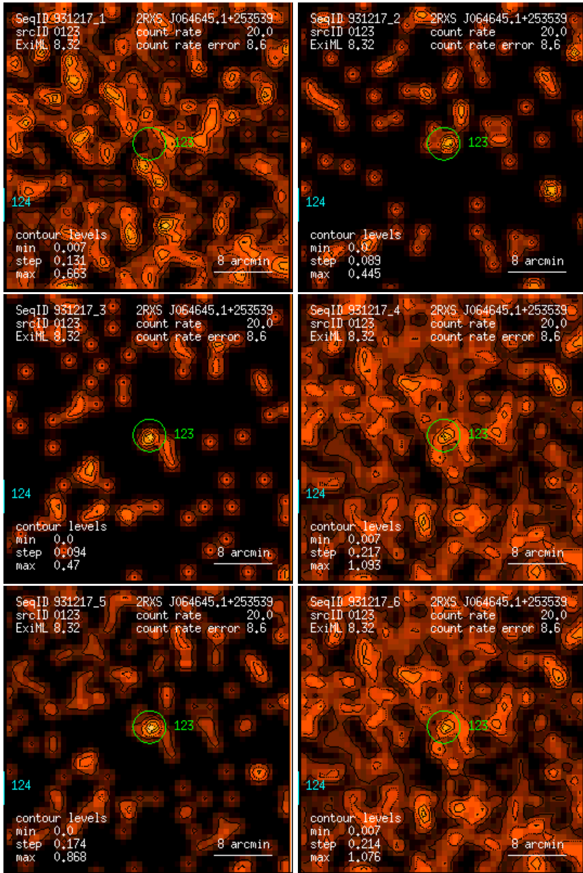
Figure 123: RASS 931217: detection 0123: band rate images, Gaussian filter: (1) PSPC channels 11 – 41, (2) 52 – 90, (3) 91 – 201, (4) 11 – 235, (5) 52 – 201, (6) 11 – 201. Broad band rates in counts/ks. Band rate contour levels in counts/ks/arcmin 2 .
