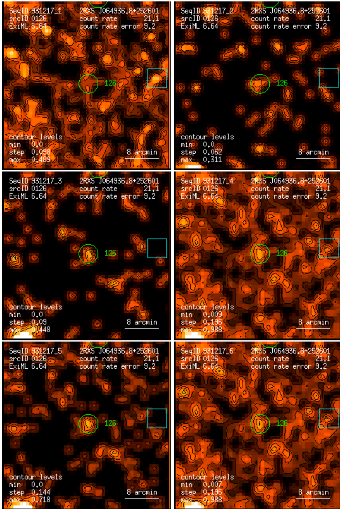
Figure 126: RASS 931217: detection 0126: band rate images, Gaussian filter: (1) PSPC channels 11 – 41, (2) 52 – 90, (3) 91 – 201, (4) 11 – 235, (5) 52 – 201, (6) 11 – 201. Broad band rates in counts/ks. Band rate contour levels in counts/ks/arcmin 2 .
