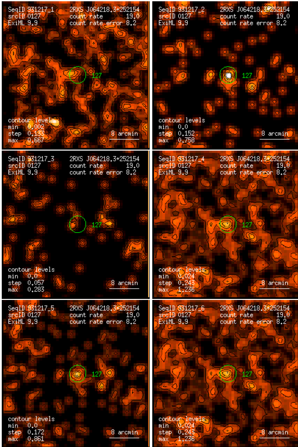
Figure 127: RASS 931217: detection 0127: band rate images, Gaussian filter: (1) PSPC channels 11 – 41, (2) 52 – 90, (3) 91 – 201, (4) 11 – 235, (5) 52 – 201, (6) 11 – 201. Broad band rates in counts/ks. Band rate contour levels in counts/ks/arcmin 2 .
