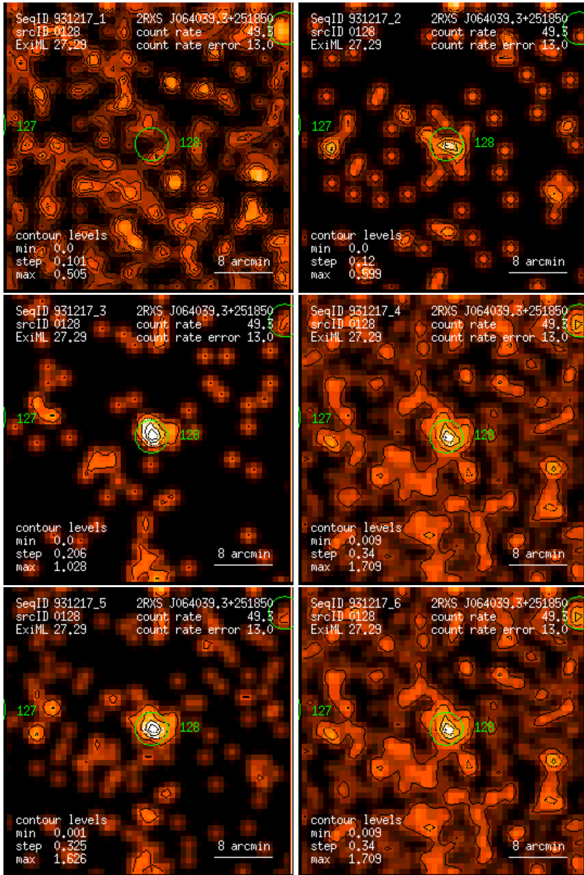
Figure 128: RASS 931217: detection 0128: band rate images, Gaussian filter: (1) PSPC channels 11 – 41, (2) 52 – 90, (3) 91 – 201, (4) 11 – 235, (5) 52 – 201, (6) 11 – 201. Broad band rates in counts/ks. Band rate contour levels in counts/ks/arcmin 2 .
