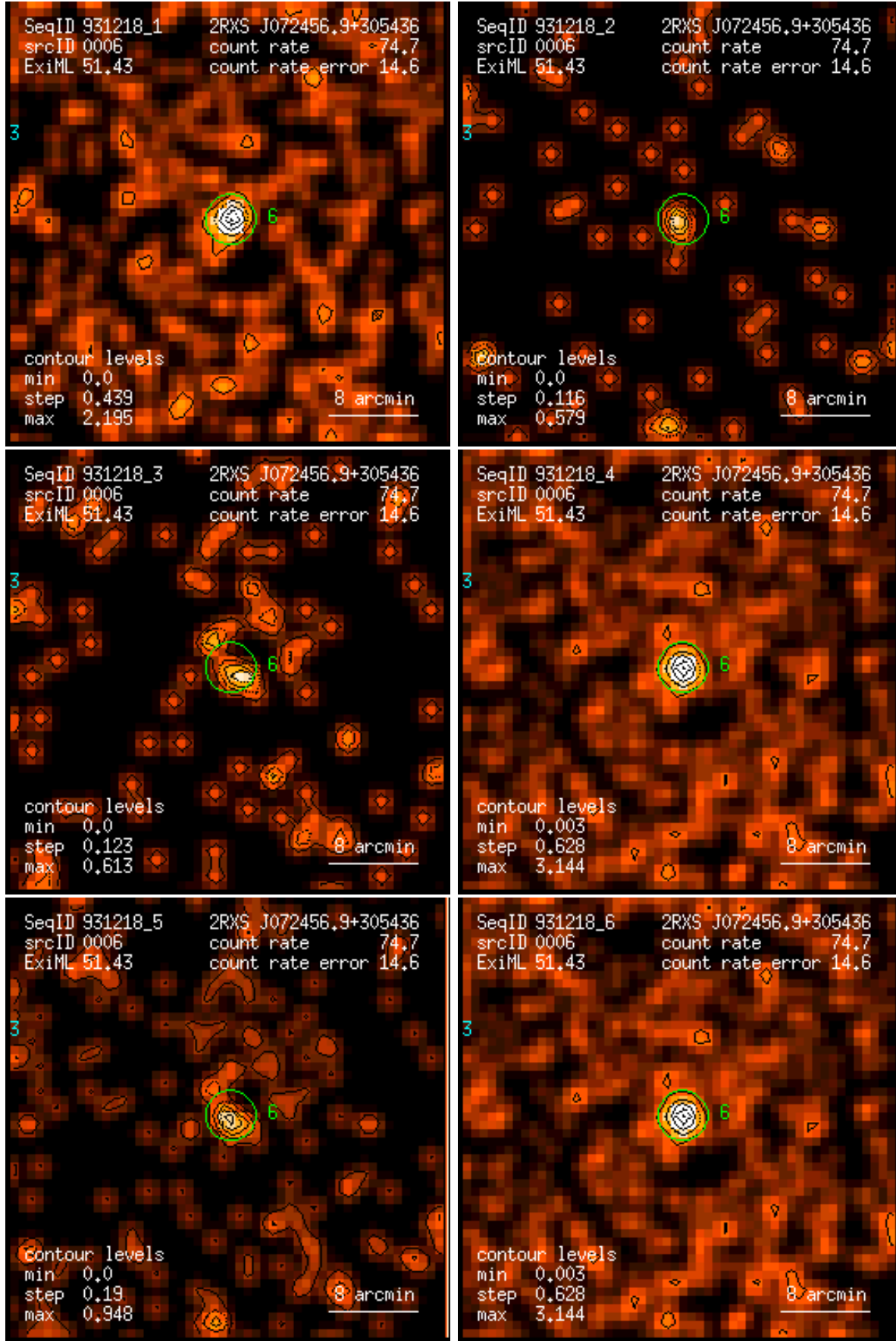
Figure 6: RASS 931218: detection 0006: band rate images, Gaussian filter: (1) PSPC channels 11 – 41, (2) 52 – 90, (3) 91 – 201, (4) 11 – 235, (5) 52 – 201, (6) 11 – 201. Broad band rates in counts/ks. Band rate contour levels in counts/ks/arcmin 2 .
