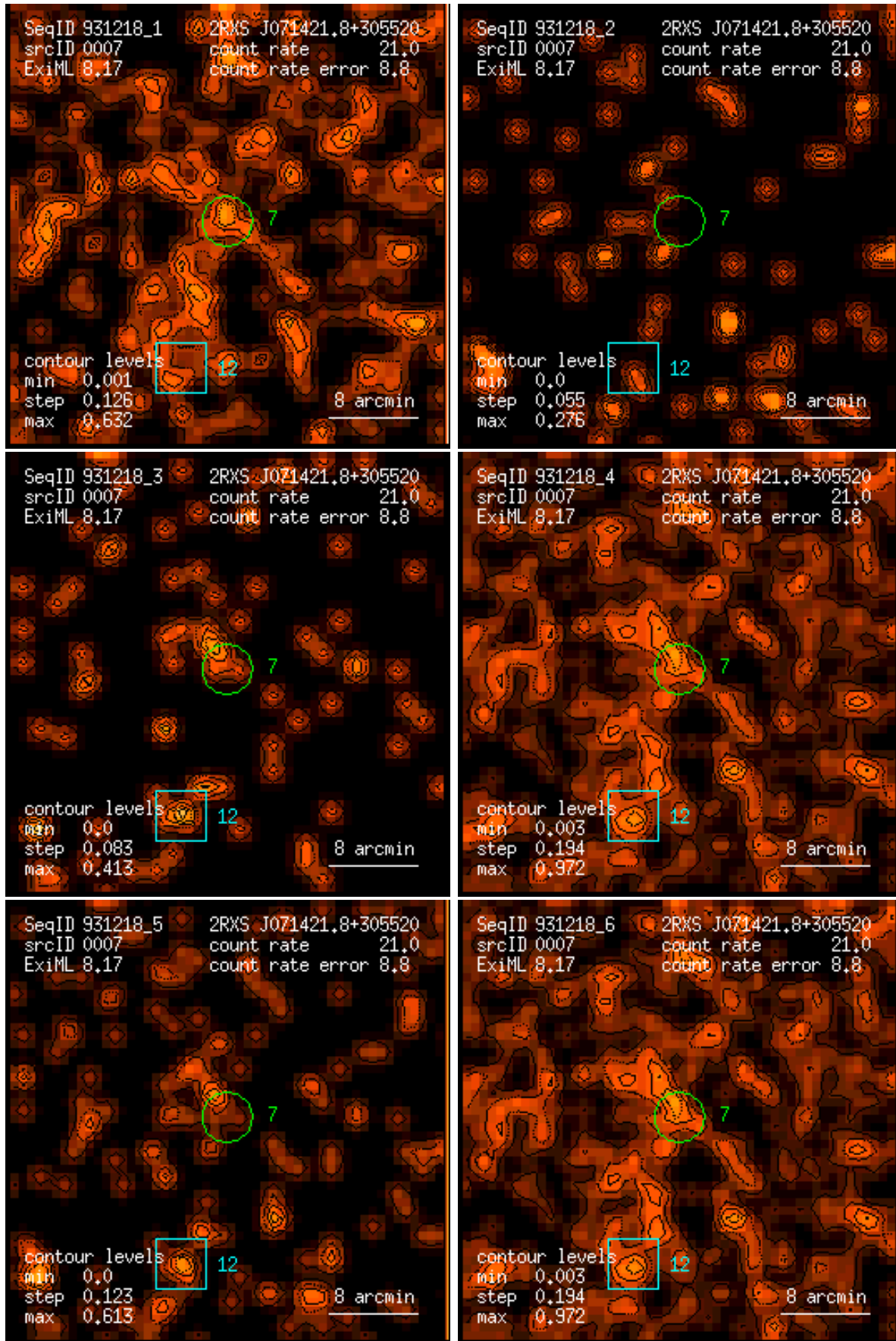
Figure 7: RASS 931218: detection 0007: band rate images, Gaussian filter: (1) PSPC channels 11 – 41, (2) 52 – 90, (3) 91 – 201, (4) 11 – 235, (5) 52 – 201, (6) 11 – 201. Broad band rates in counts/ks. Band rate contour levels in counts/ks/arcmin 2 .
