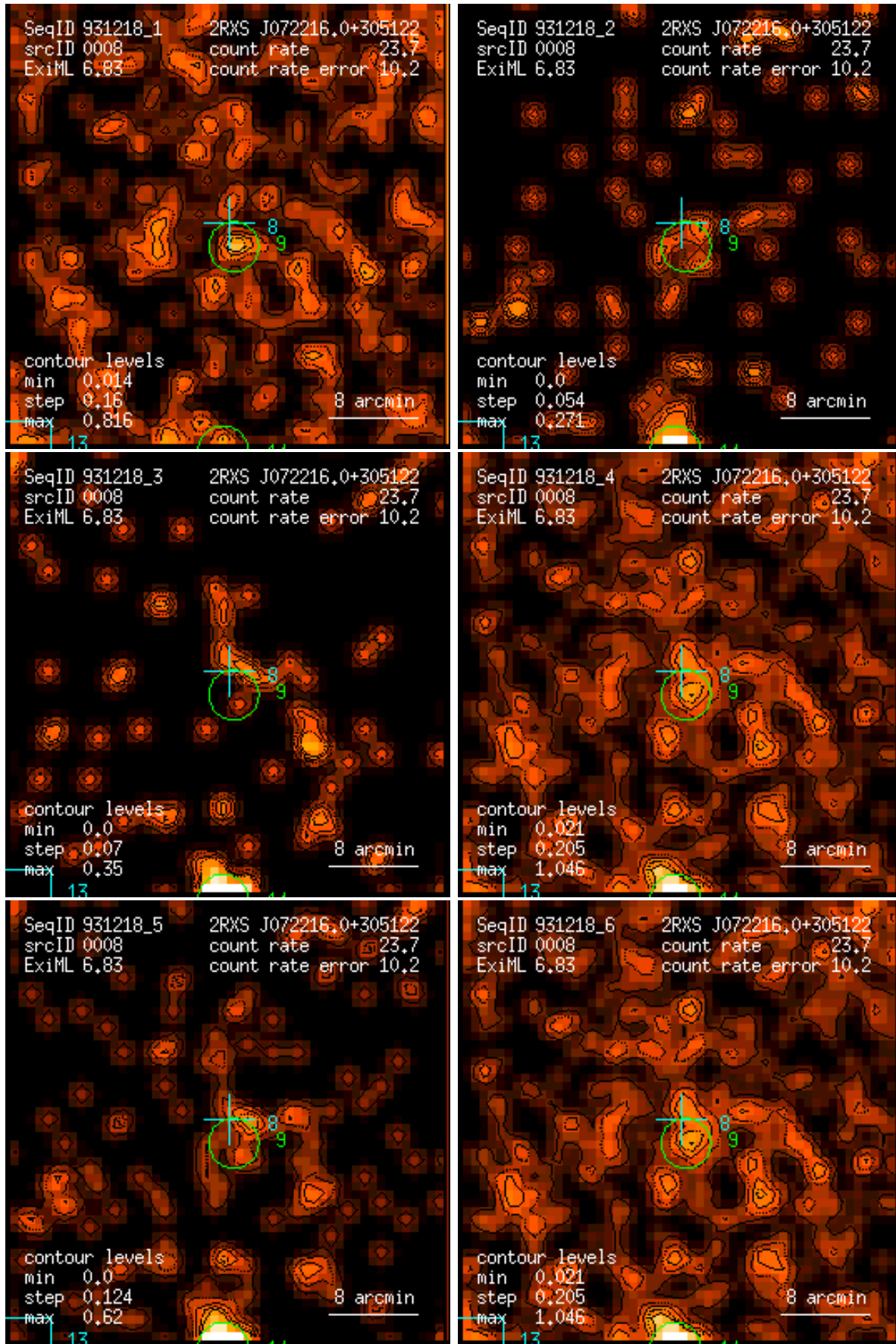
Figure 8: RASS 931218: detection 0008: band rate images, Gaussian filter: (1) PSPC channels 11 – 41, (2) 52 – 90, (3) 91 – 201, (4) 11 – 235, (5) 52 – 201, (6) 11 – 201. Broad band rates in counts/ks. Band rate contour levels in counts/ks/arcmin 2 .
