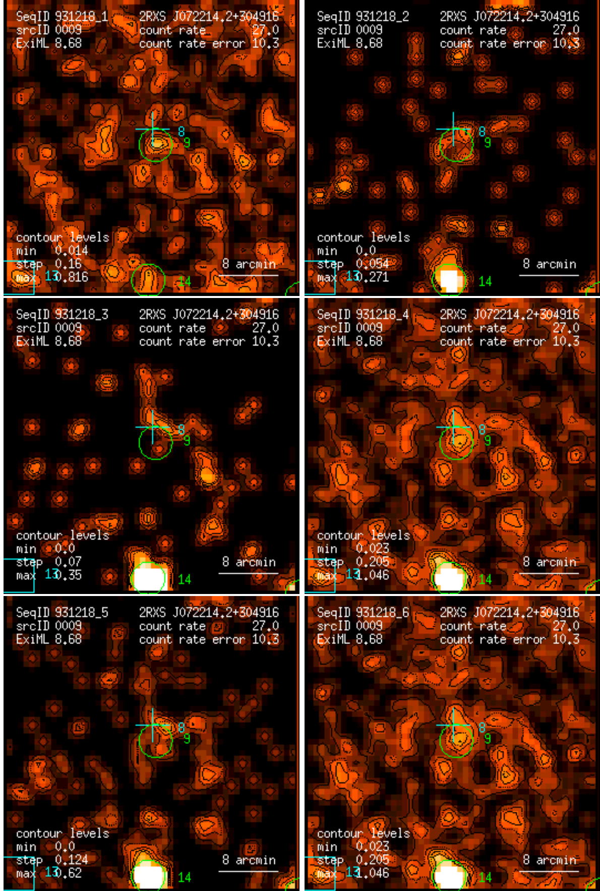
Figure 9: RASS 931218: detection 0009: band rate images, Gaussian filter: (1) PSPC channels 11 – 41, (2) 52 – 90, (3) 91 – 201, (4) 11 – 235, (5) 52 – 201, (6) 11 – 201. Broad band rates in counts/ks. Band rate contour levels in counts/ks/arcmin 2 .
