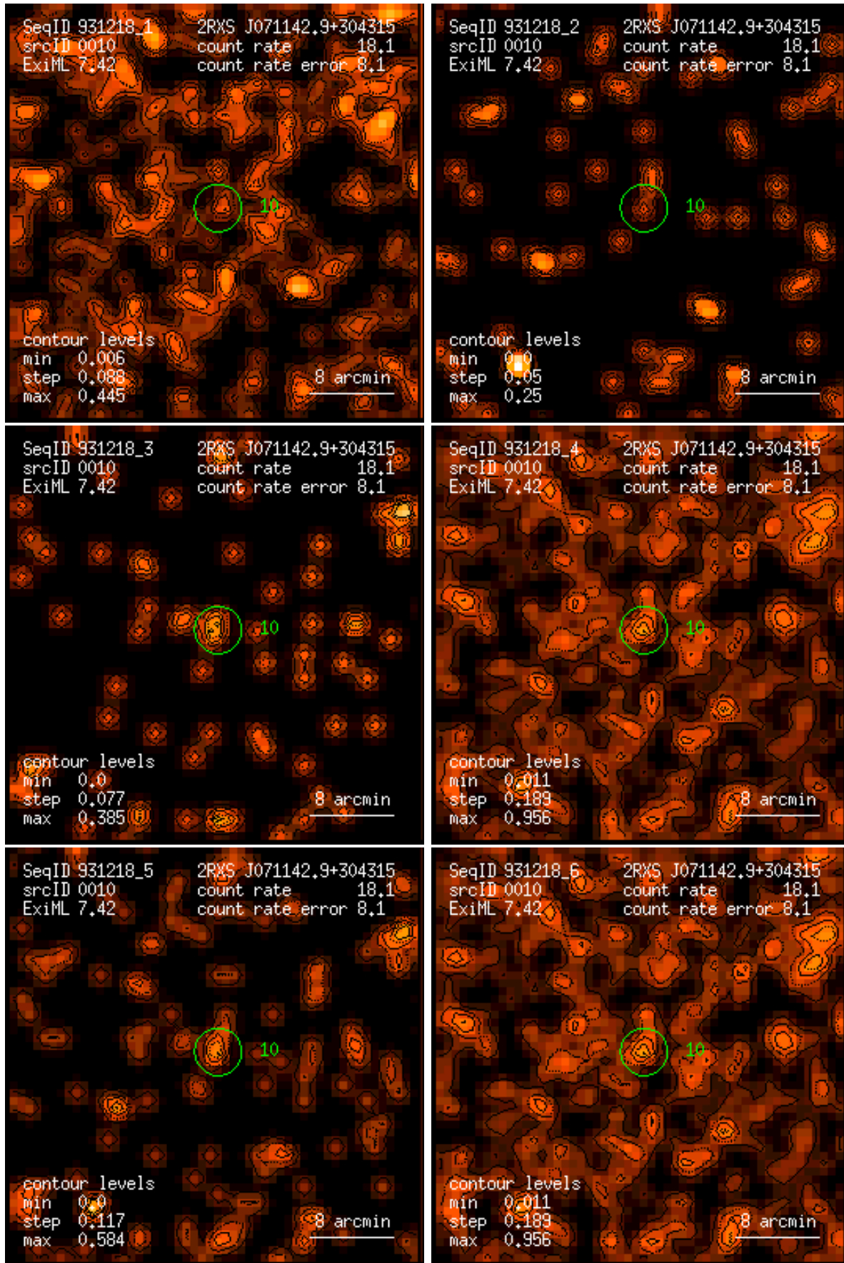
Figure 10: RASS 931218: detection 0010: band rate images, Gaussian filter: (1) PSPC channels 11 – 41, (2) 52 – 90, (3) 91 – 201, (4) 11 – 235, (5) 52 – 201, (6) 11 – 201. Broad band rates in counts/ks. Band rate contour levels in counts/ks/arcmin 2 .
