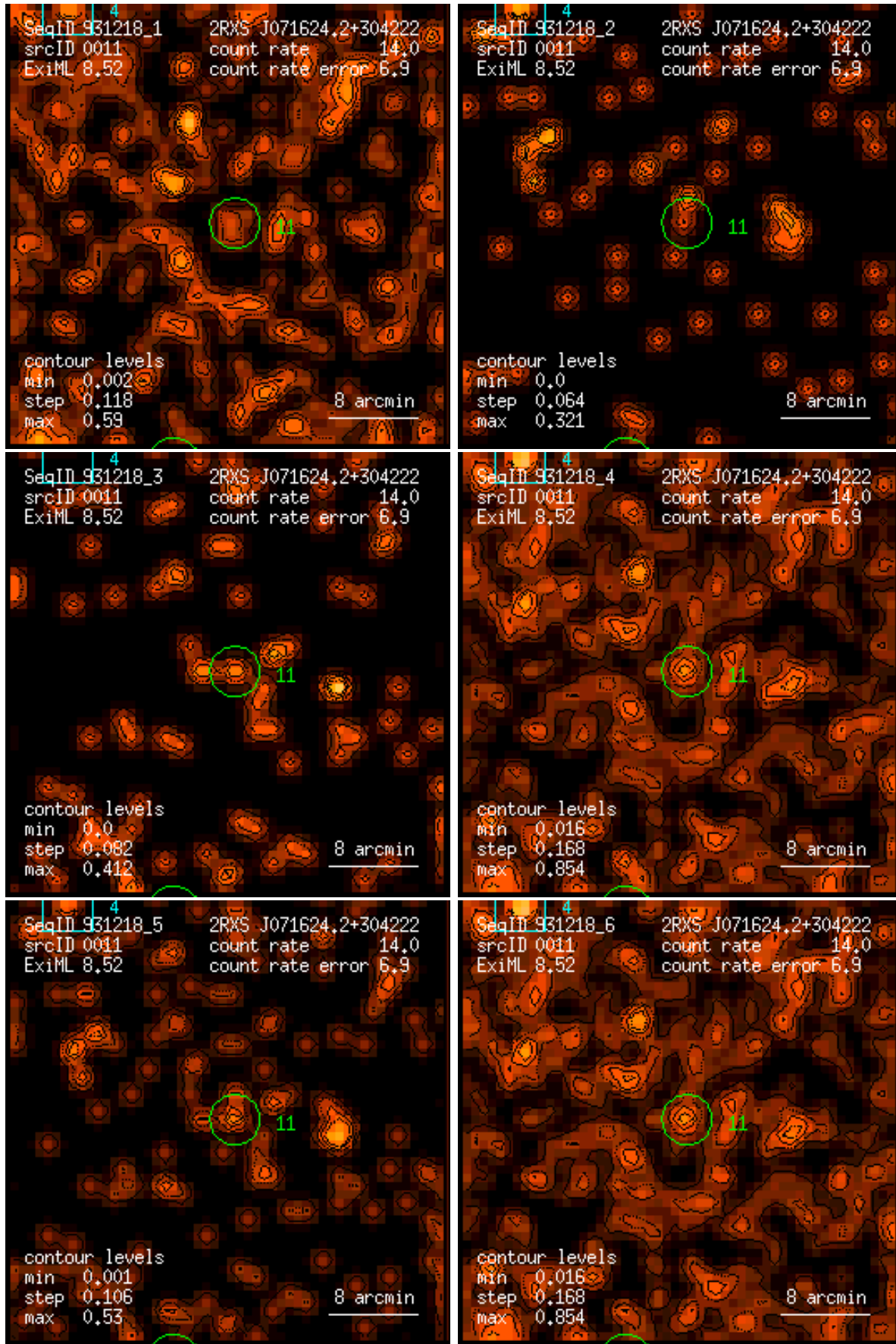
Figure 11: RASS 931218: detection 0011: band rate images, Gaussian filter: (1) PSPC channels 11 – 41, (2) 52 – 90, (3) 91 – 201, (4) 11 – 235, (5) 52 – 201, (6) 11 – 201. Broad band rates in counts/ks. Band rate contour levels in counts/ks/arcmin 2 .
