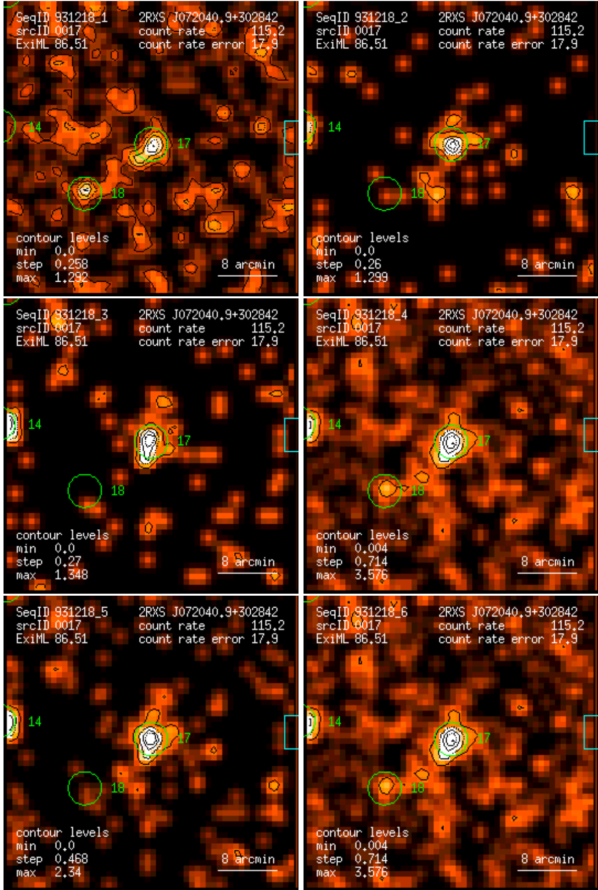
Figure 17: RASS 931218: detection 0017: band rate images, Gaussian filter: (1) PSPC channels 11 – 41, (2) 52 – 90, (3) 91 – 201, (4) 11 – 235, (5) 52 – 201, (6) 11 – 201. Broad band rates in counts/ks. Band rate contour levels in counts/ks/arcmin 2 .
