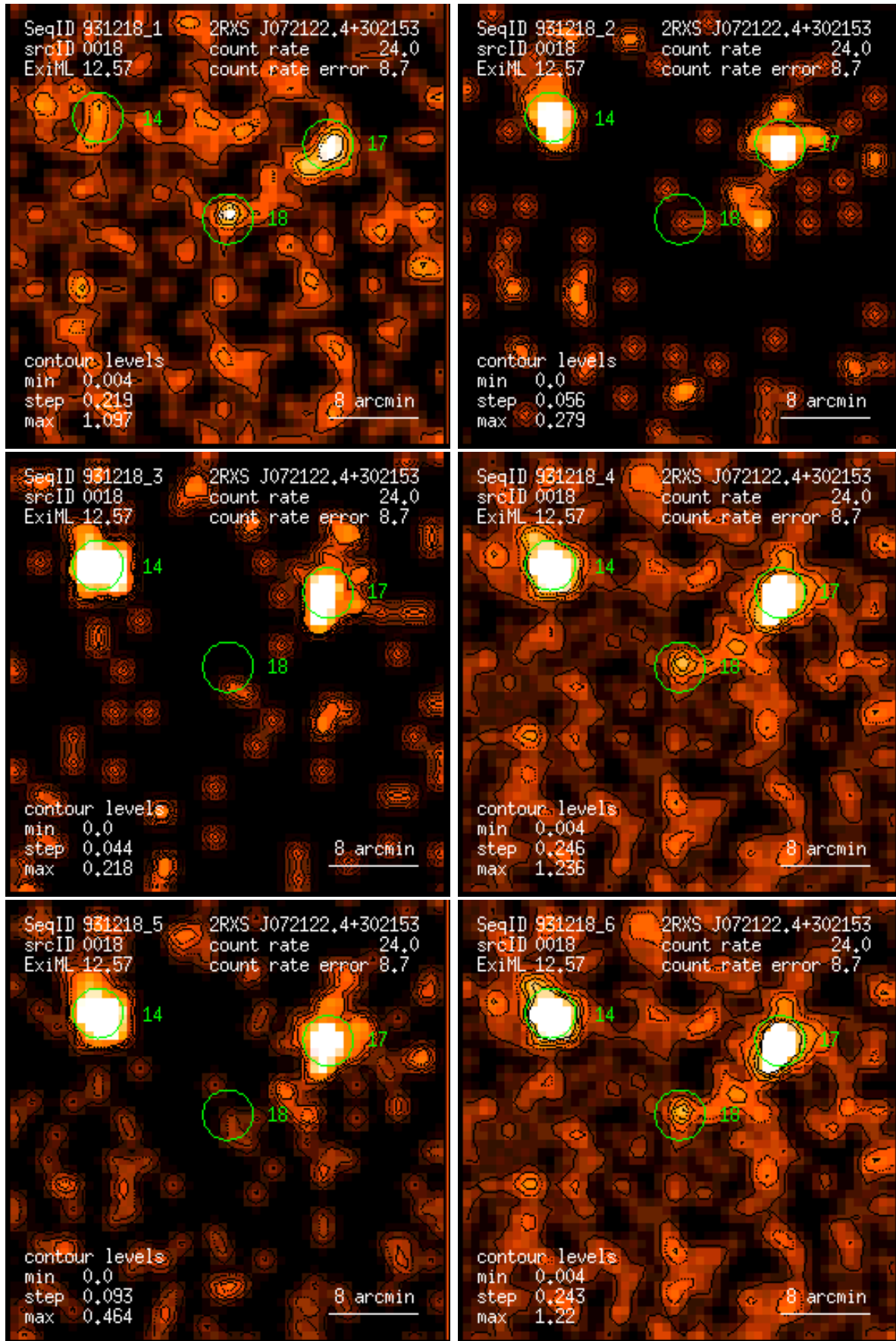
Figure 18: RASS 931218: detection 0018: band rate images, Gaussian filter: (1) PSPC channels 11 – 41, (2) 52 – 90, (3) 91 – 201, (4) 11 – 235, (5) 52 – 201, (6) 11 – 201. Broad band rates in counts/ks. Band rate contour levels in counts/ks/arcmin 2 .
