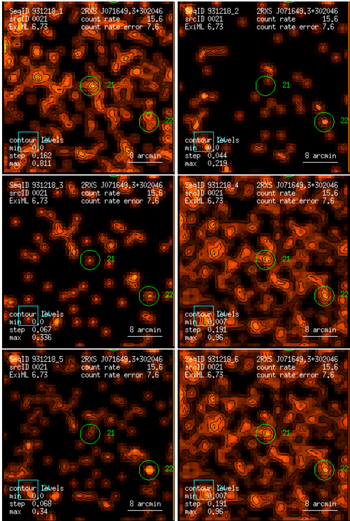
Figure 21: RASS 931218: detection 0021: band rate images, Gaussian filter: (1) PSPC channels 11 – 41, (2) 52 – 90, (3) 91 – 201, (4) 11 – 235, (5) 52 – 201, (6) 11 – 201. Broad band rates in counts/ks. Band rate contour levels in counts/ks/arcmin 2 .
