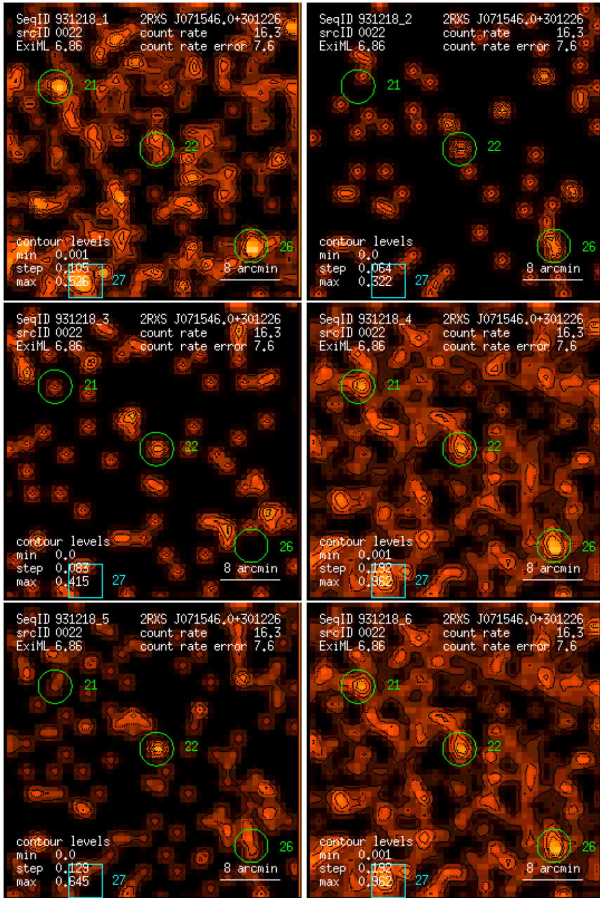
Figure 22: RASS 931218: detection 0022: band rate images, Gaussian filter: (1) PSPC channels 11 – 41, (2) 52 – 90, (3) 91 – 201, (4) 11 – 235, (5) 52 – 201, (6) 11 – 201. Broad band rates in counts/ks. Band rate contour levels in counts/ks/arcmin 2 .
