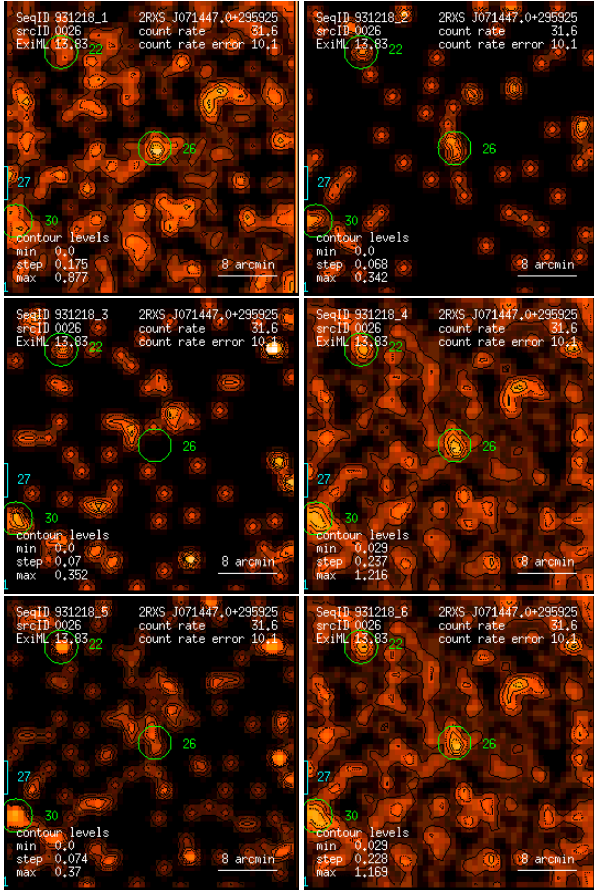
Figure 26: RASS 931218: detection 0026: band rate images, Gaussian filter: (1) PSPC channels 11 – 41, (2) 52 – 90, (3) 91 – 201, (4) 11 – 235, (5) 52 – 201, (6) 11 – 201. Broad band rates in counts/ks. Band rate contour levels in counts/ks/arcmin 2 .
