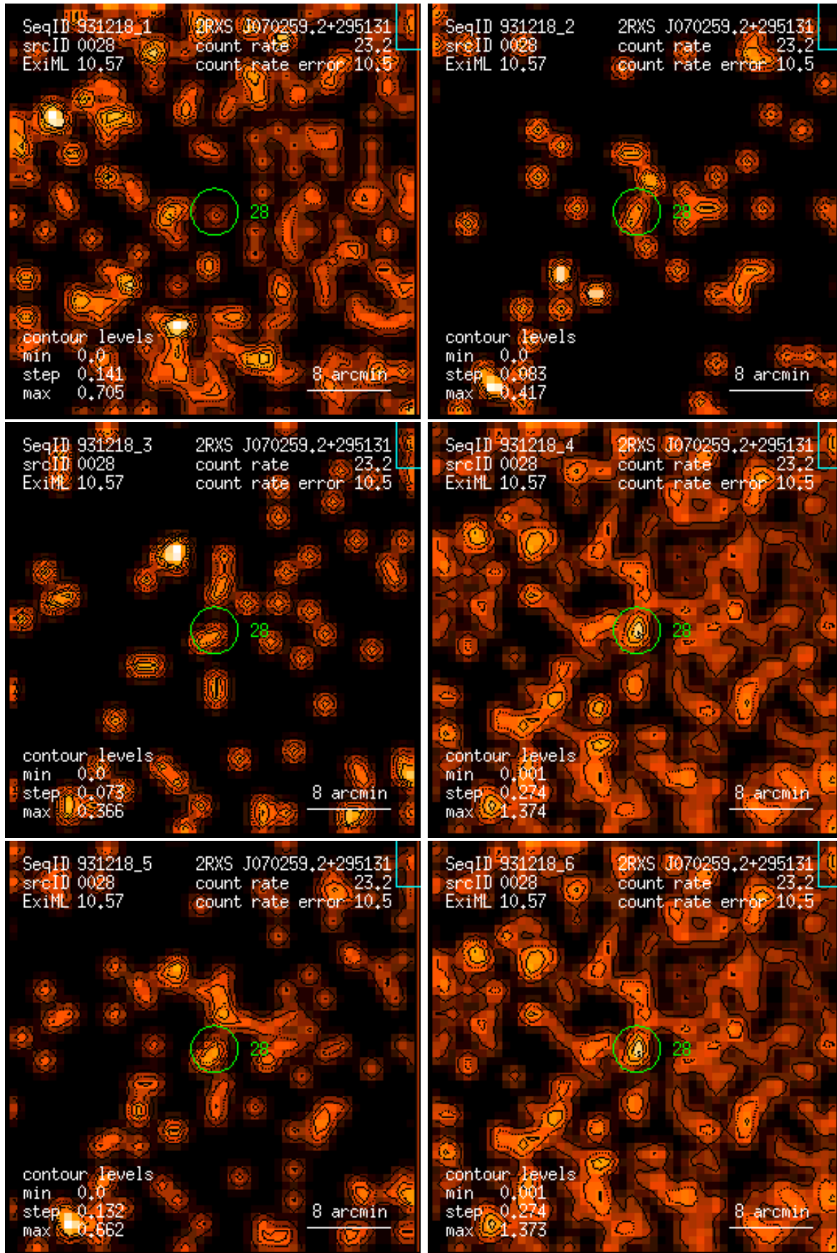
Figure 28: RASS 931218: detection 0028: band rate images, Gaussian filter: (1) PSPC channels 11 – 41, (2) 52 – 90, (3) 91 – 201, (4) 11 – 235, (5) 52 – 201, (6) 11 – 201. Broad band rates in counts/ks. Band rate contour levels in counts/ks/arcmin 2 .
