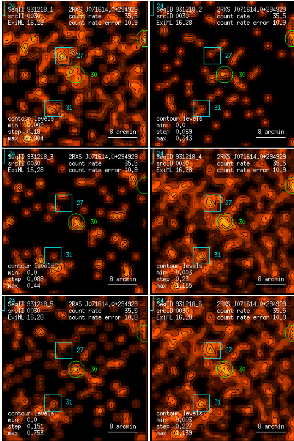
Figure 30: RASS 931218: detection 0030: band rate images, Gaussian filter: (1) PSPC channels 11 – 41, (2) 52 – 90, (3) 91 – 201, (4) 11 – 235, (5) 52 – 201, (6) 11 – 201. Broad band rates in counts/ks. Band rate contour levels in counts/ks/arcmin 2 .
