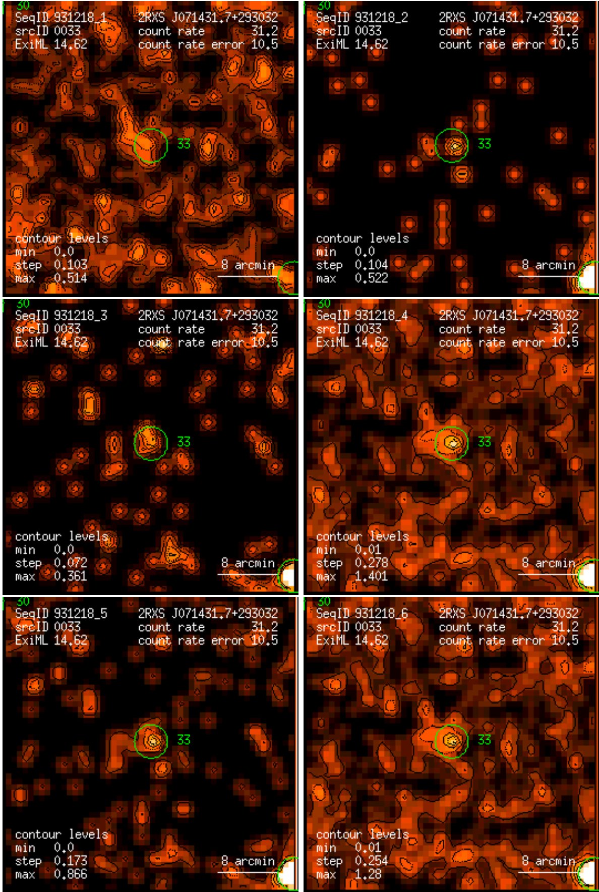
Figure 33: RASS 931218: detection 0033: band rate images, Gaussian filter: (1) PSPC channels 11 – 41, (2) 52 – 90, (3) 91 – 201, (4) 11 – 235, (5) 52 – 201, (6) 11 – 201. Broad band rates in counts/ks. Band rate contour levels in counts/ks/arcmin 2 .
