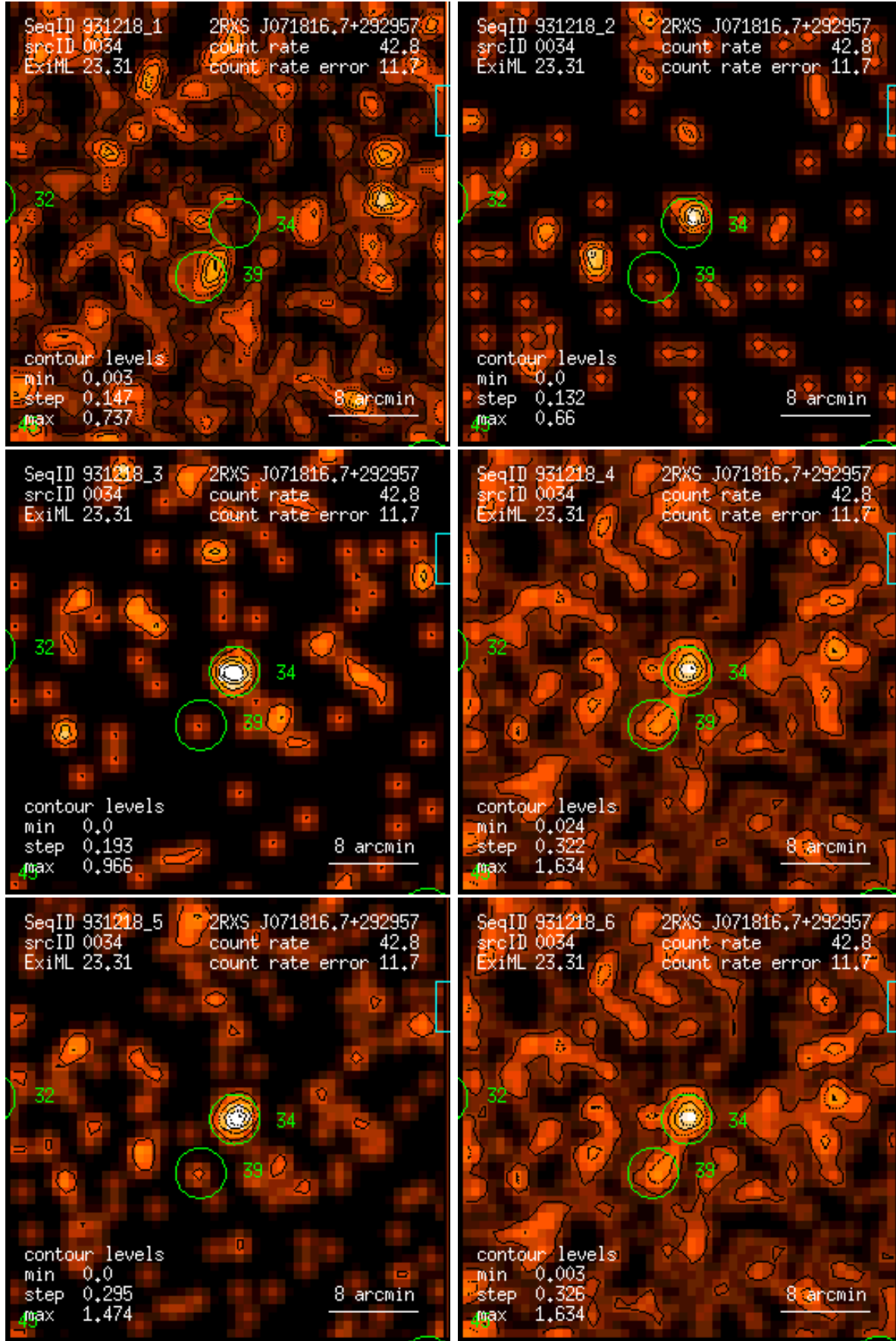
Figure 34: RASS 931218: detection 0034: band rate images, Gaussian filter: (1) PSPC channels 11 – 41, (2) 52 – 90, (3) 91 – 201, (4) 11 – 235, (5) 52 – 201, (6) 11 – 201. Broad band rates in counts/ks. Band rate contour levels in counts/ks/arcmin 2 .
