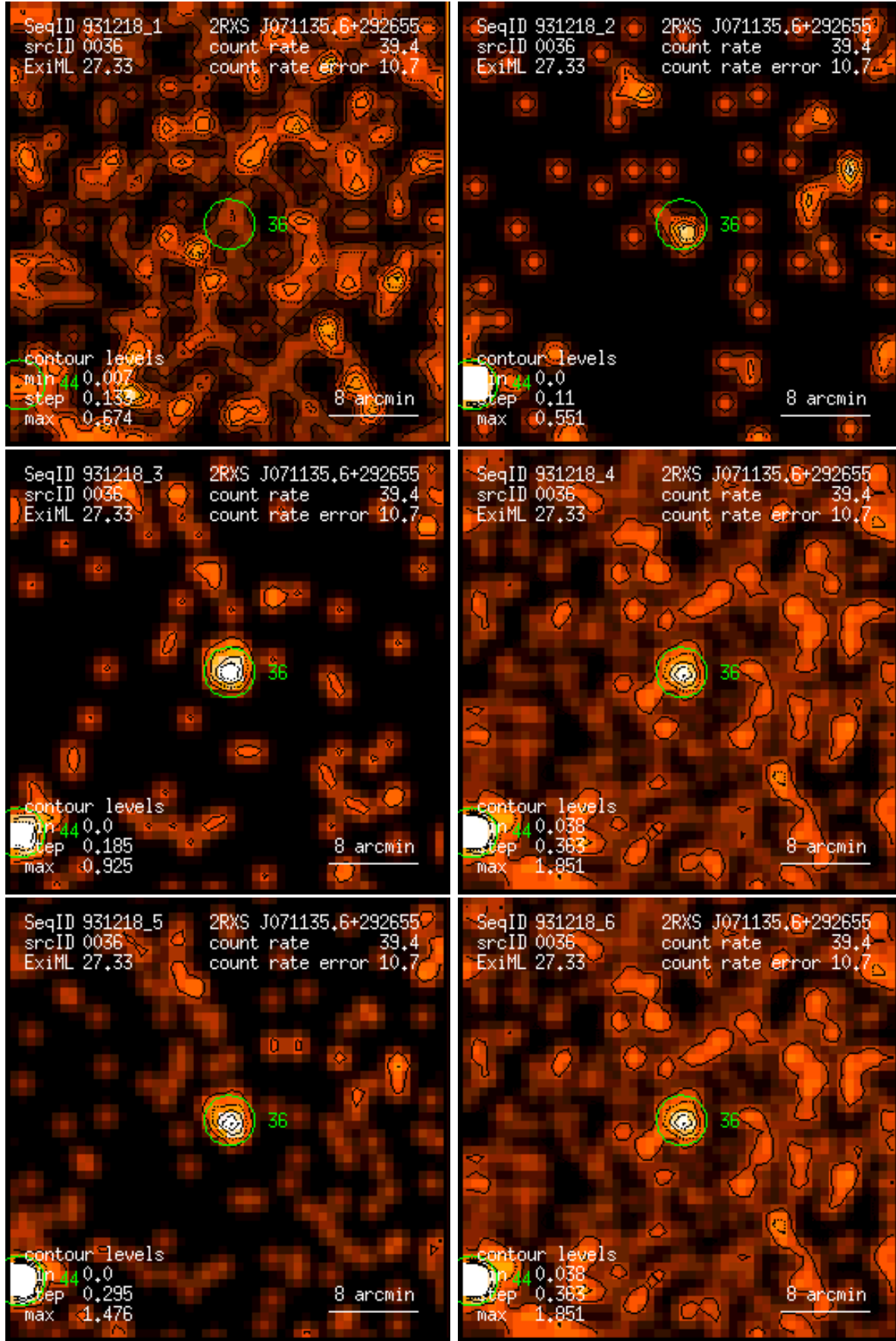
Figure 36: RASS 931218: detection 0036: band rate images, Gaussian filter: (1) PSPC channels 11 – 41, (2) 52 – 90, (3) 91 – 201, (4) 11 – 235, (5) 52 – 201, (6) 11 – 201. Broad band rates in counts/ks. Band rate contour levels in counts/ks/arcmin 2 .
