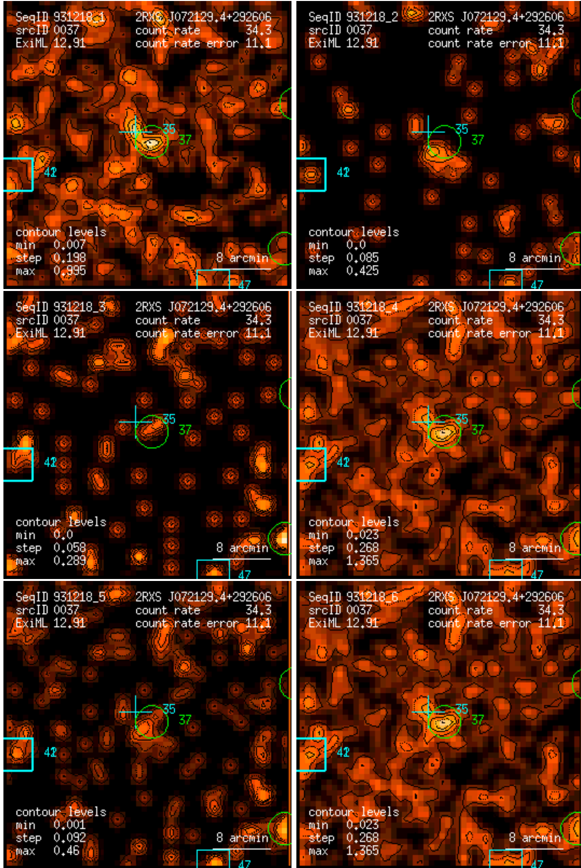
Figure 37: RASS 931218: detection 0037: band rate images, Gaussian filter: (1) PSPC channels 11 – 41, (2) 52 – 90, (3) 91 – 201, (4) 11 – 235, (5) 52 – 201, (6) 11 – 201. Broad band rates in counts/ks. Band rate contour levels in counts/ks/arcmin 2 .
