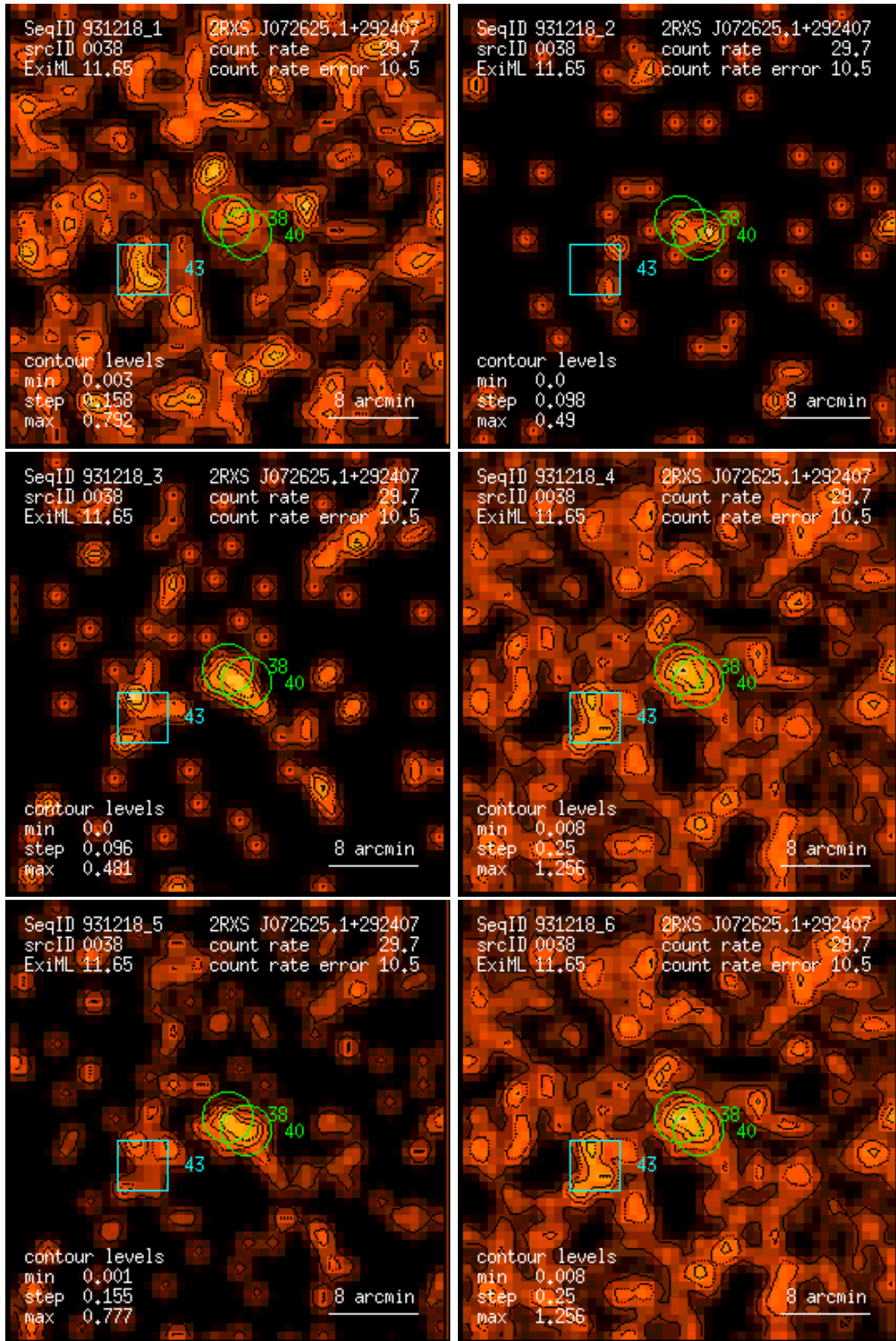
Figure 38: RASS 931218: detection 0038: band rate images, Gaussian filter: (1) PSPC channels 11 – 41, (2) 52 – 90, (3) 91 – 201, (4) 11 – 235, (5) 52 – 201, (6) 11 – 201. Broad band rates in counts/ks. Band rate contour levels in counts/ks/arcmin 2 .
