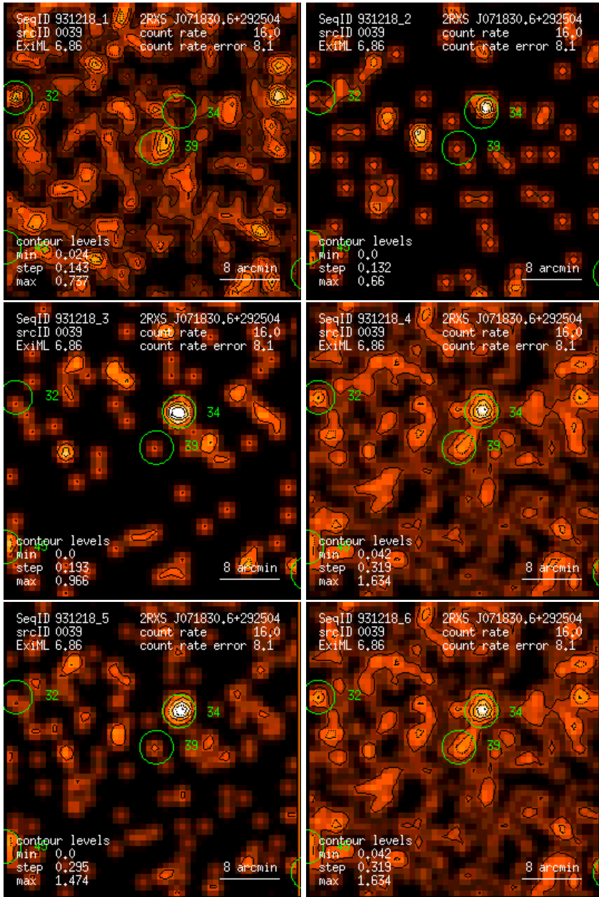
Figure 39: RASS 931218: detection 0039: band rate images, Gaussian filter: (1) PSPC channels 11 – 41, (2) 52 – 90, (3) 91 – 201, (4) 11 – 235, (5) 52 – 201, (6) 11 – 201. Broad band rates in counts/ks. Band rate contour levels in counts/ks/arcmin 2 .
