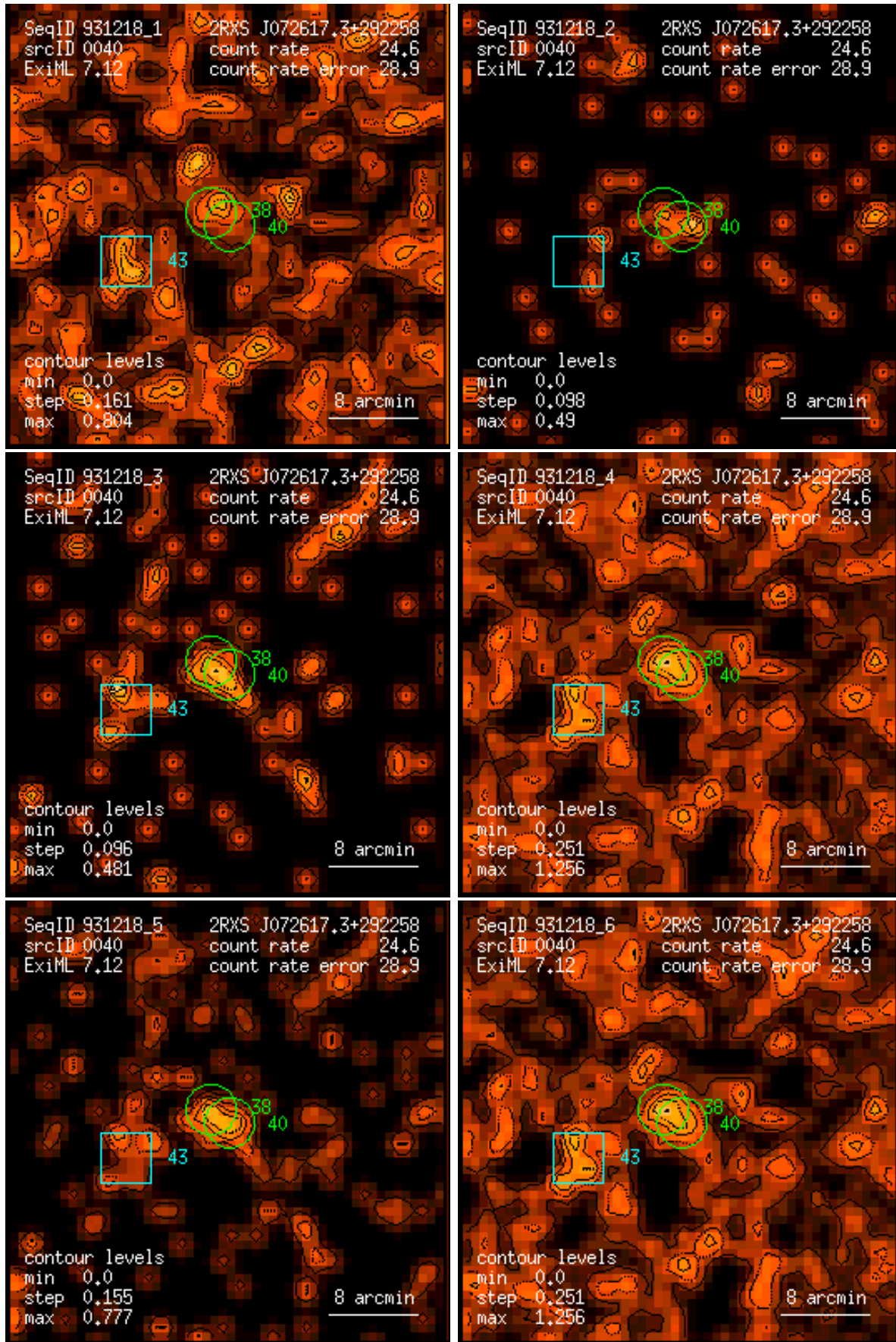
Figure 40: RASS 931218: detection 0040: band rate images, Gaussian filter: (1) PSPC channels 11 – 41, (2) 52 – 90, (3) 91 – 201, (4) 11 – 235, (5) 52 – 201, (6) 11 – 201. Broad band rates in counts/ks. Band rate contour levels in counts/ks/arcmin 2 .
