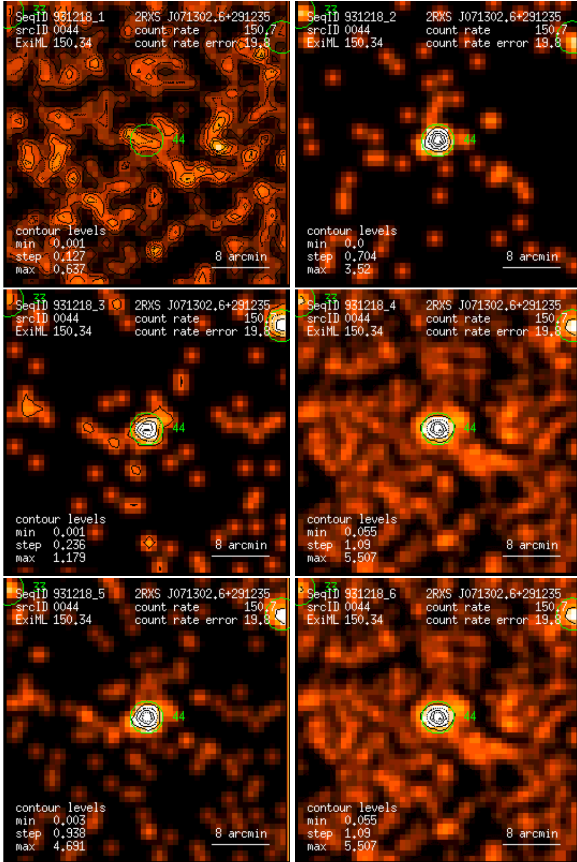
Figure 44: RASS 931218: detection 0044: band rate images, Gaussian filter: (1) PSPC channels 11 – 41, (2) 52 – 90, (3) 91 – 201, (4) 11 – 235, (5) 52 – 201, (6) 11 – 201. Broad band rates in counts/ks. Band rate contour levels in counts/ks/arcmin 2 .
