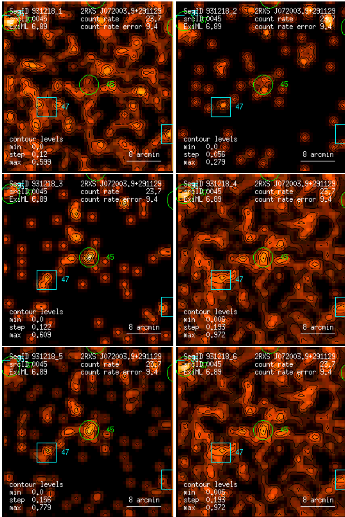
Figure 45: RASS 931218: detection 0045: band rate images, Gaussian filter: (1) PSPC channels 11 – 41, (2) 52 – 90, (3) 91 – 201, (4) 11 – 235, (5) 52 – 201, (6) 11 – 201. Broad band rates in counts/ks. Band rate contour levels in counts/ks/arcmin 2 .
