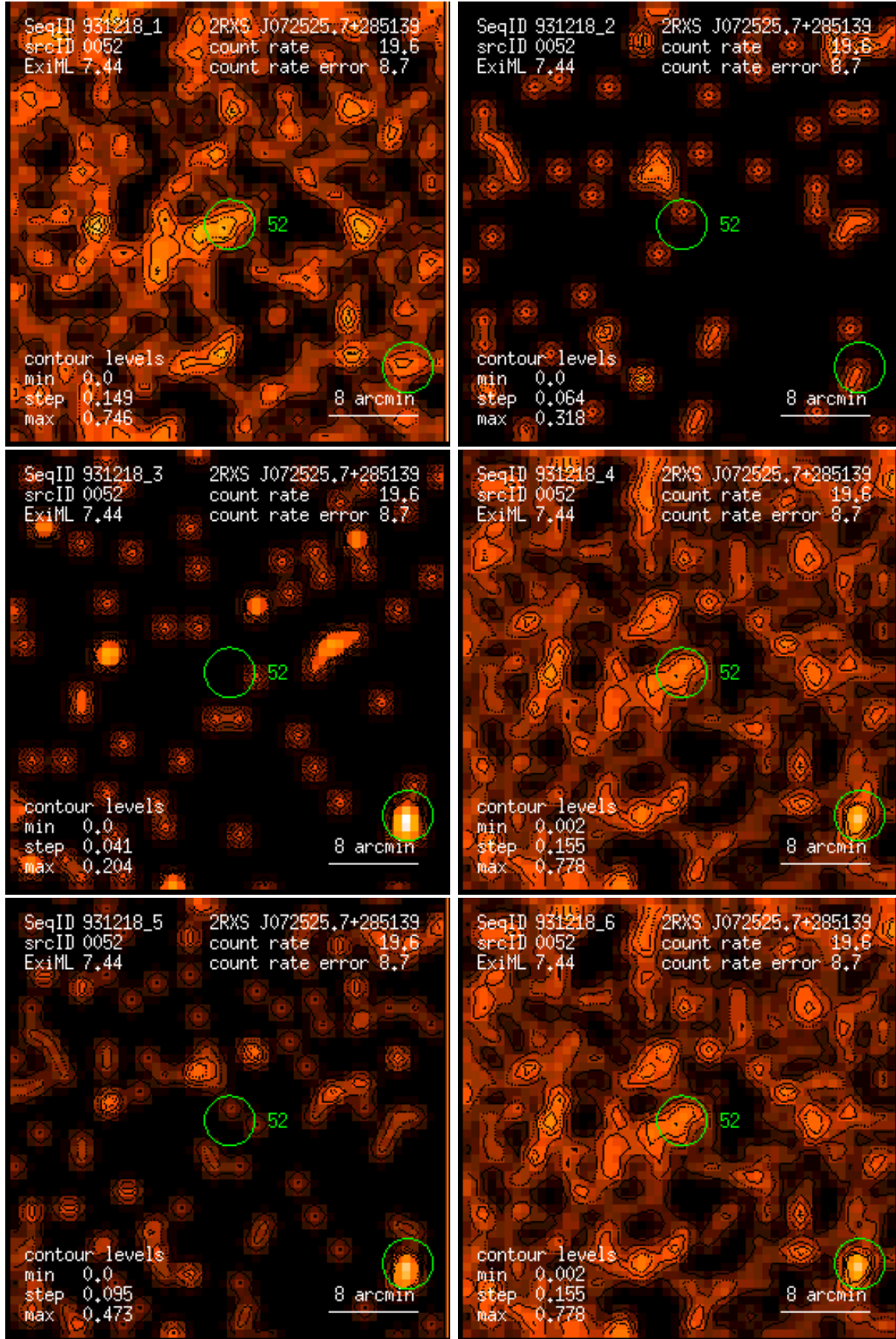
Figure 52: RASS 931218: detection 0052: band rate images, Gaussian filter: (1) PSPC channels 11 – 41, (2) 52 – 90, (3) 91 – 201, (4) 11 – 235, (5) 52 – 201, (6) 11 – 201. Broad band rates in counts/ks. Band rate contour levels in counts/ks/arcmin 2 .
