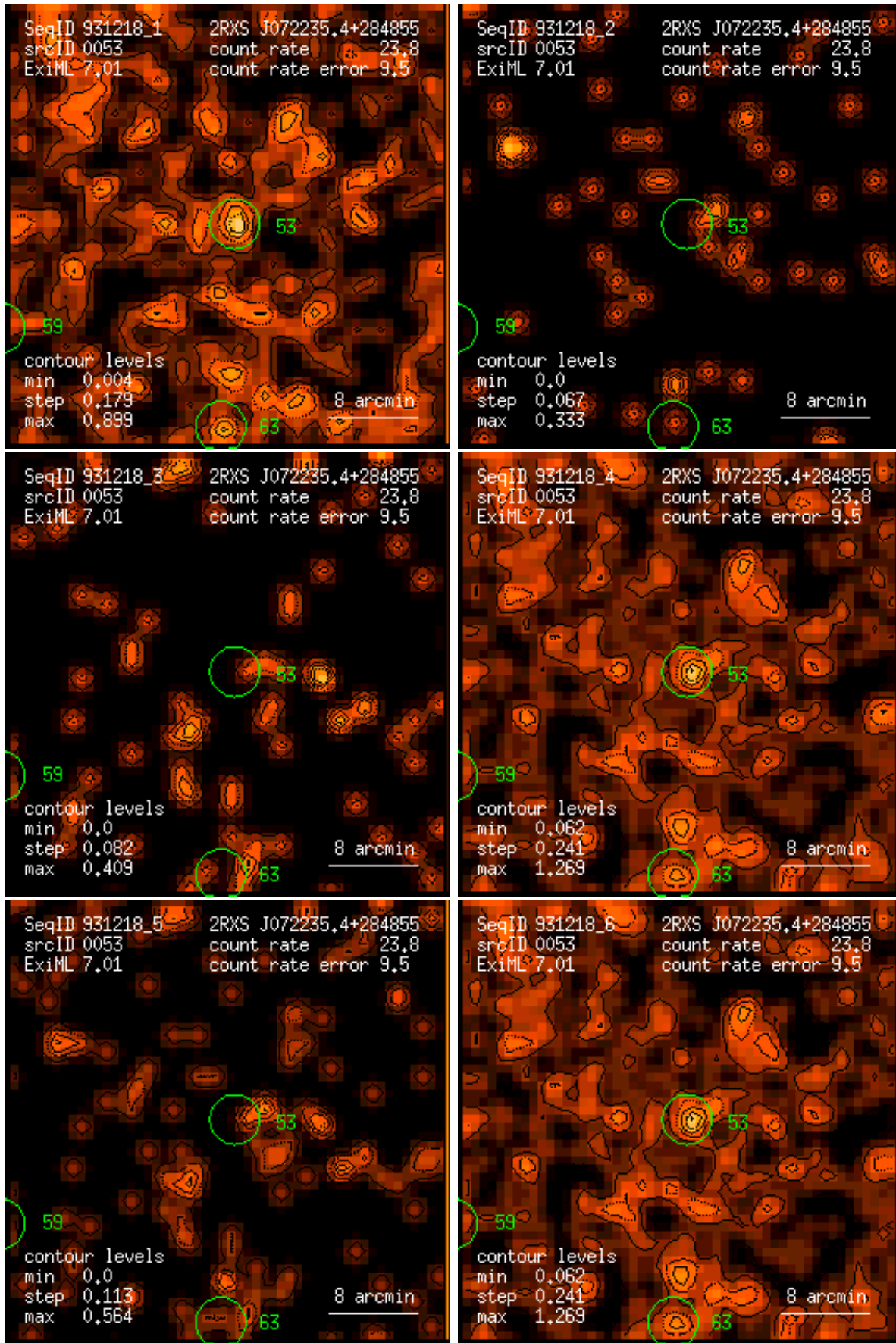
Figure 53: RASS 931218: detection 0053: band rate images, Gaussian filter: (1) PSPC channels 11 – 41, (2) 52 – 90, (3) 91 – 201, (4) 11 – 235, (5) 52 – 201, (6) 11 – 201. Broad band rates in counts/ks. Band rate contour levels in counts/ks/arcmin 2 .
