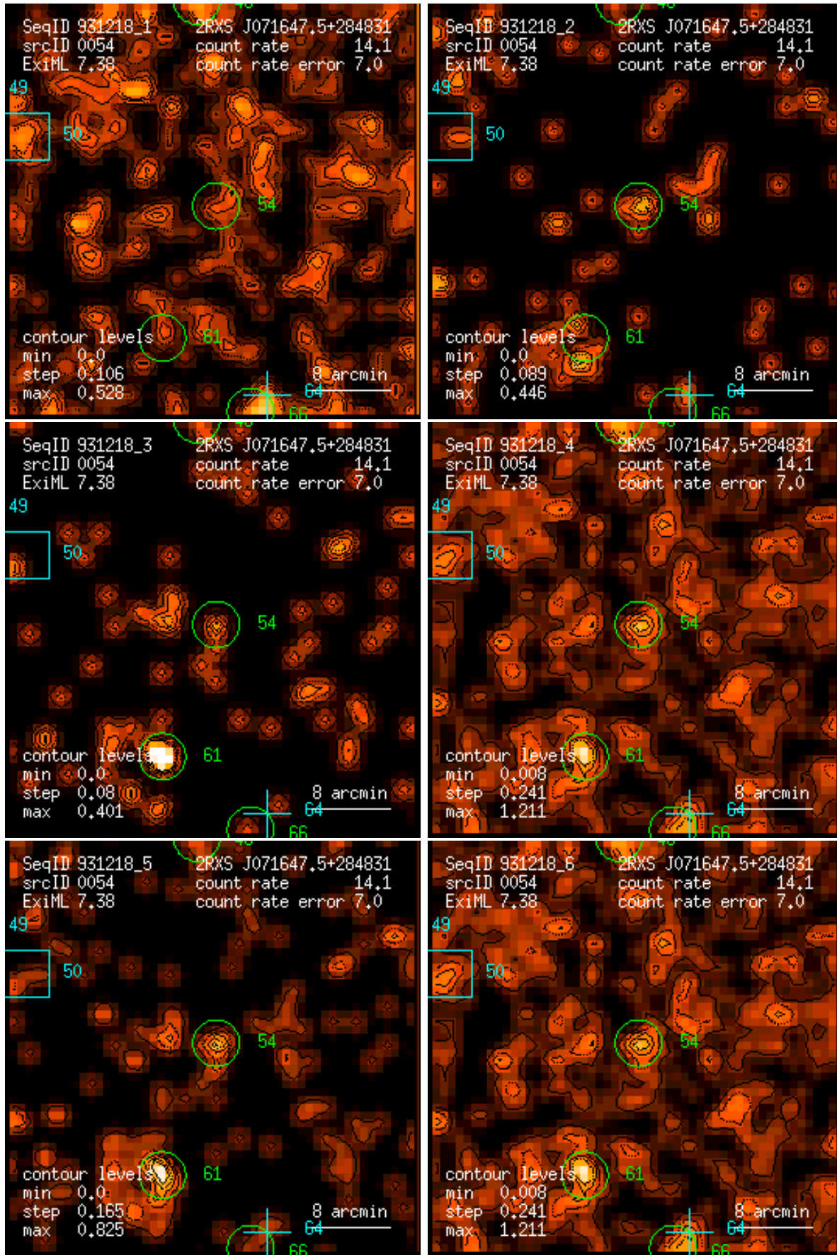
Figure 54: RASS 931218: detection 0054: band rate images, Gaussian filter: (1) PSPC channels 11 – 41, (2) 52 – 90, (3) 91 – 201, (4) 11 – 235, (5) 52 – 201, (6) 11 – 201. Broad band rates in counts/ks. Band rate contour levels in counts/ks/arcmin 2 .
