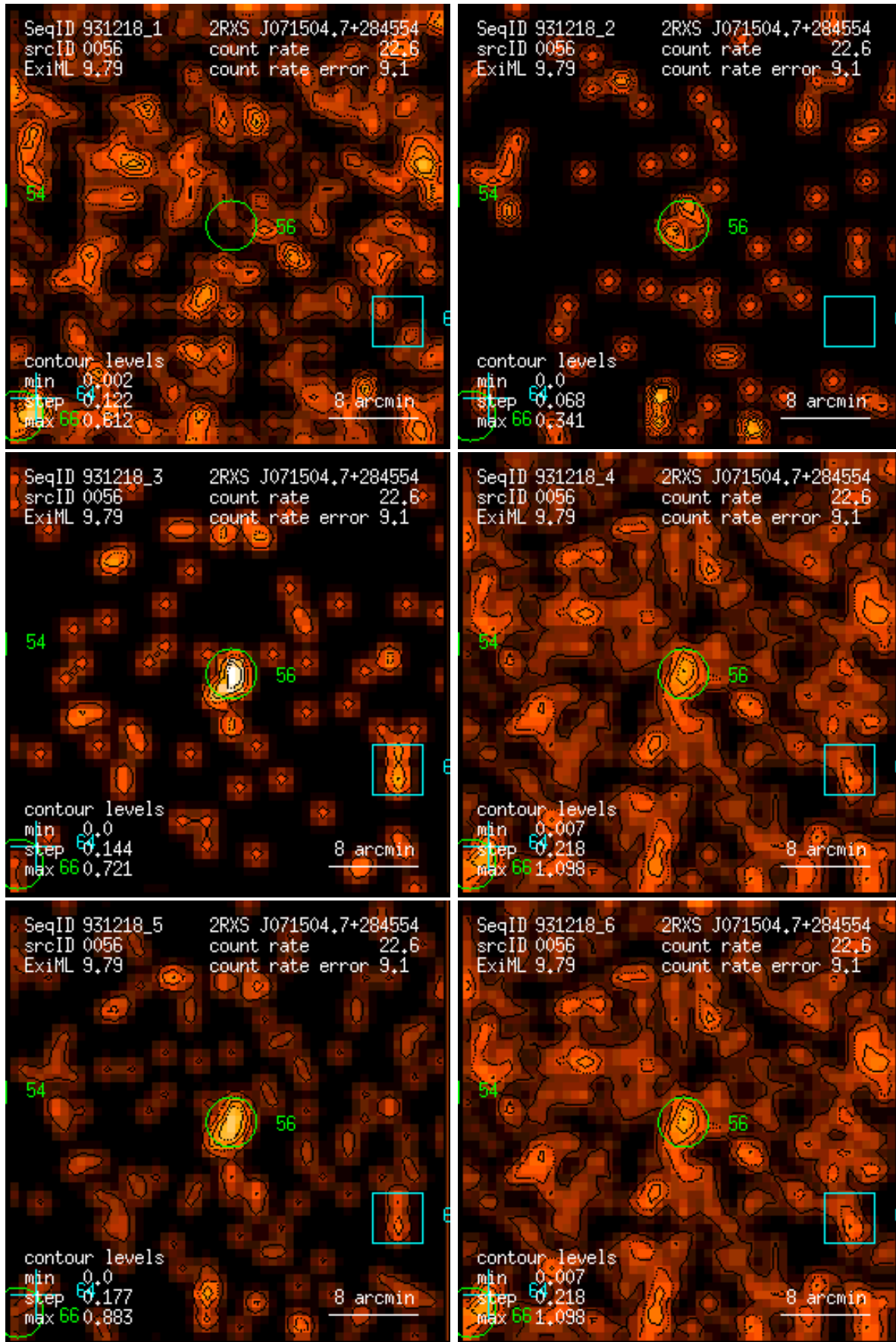
Figure 56: RASS 931218: detection 0056: band rate images, Gaussian filter: (1) PSPC channels 11 – 41, (2) 52 – 90, (3) 91 – 201, (4) 11 – 235, (5) 52 – 201, (6) 11 – 201. Broad band rates in counts/ks. Band rate contour levels in counts/ks/arcmin 2 .
