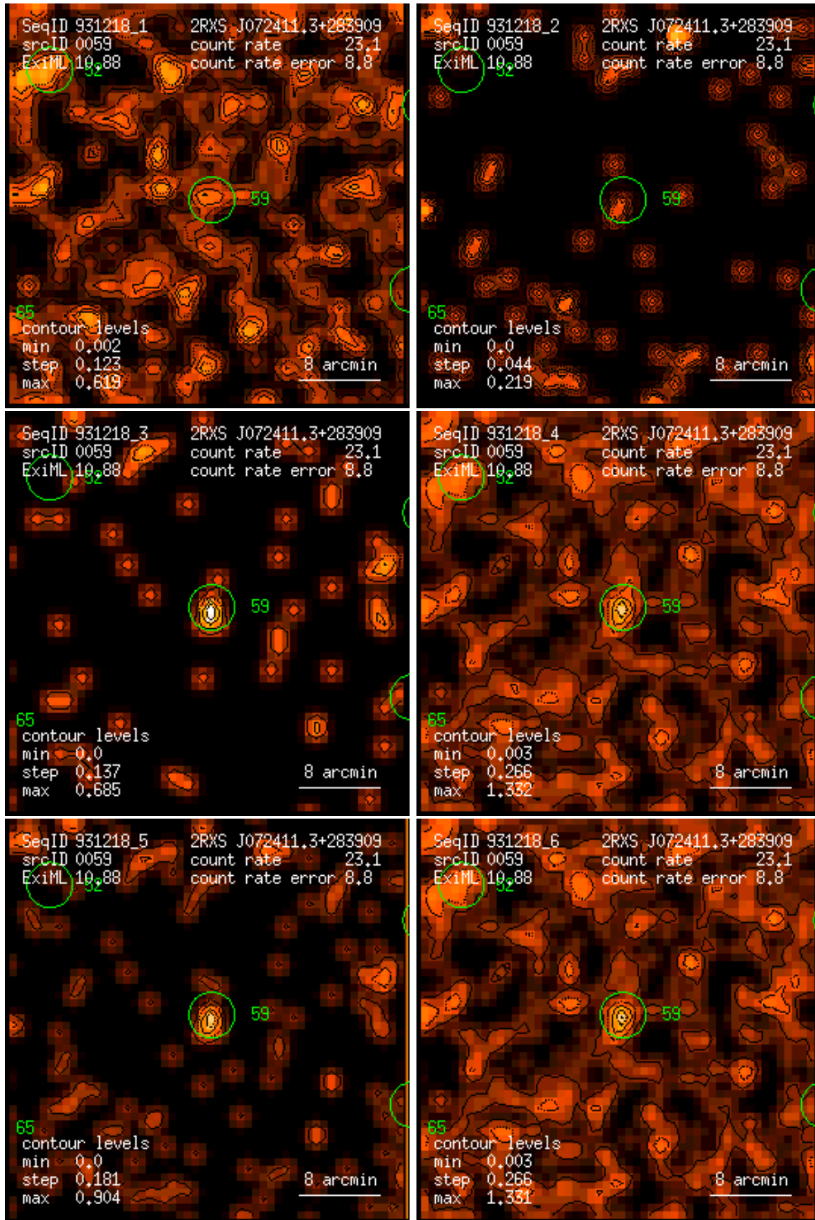
Figure 59: RASS 931218: detection 0059: band rate images, Gaussian filter: (1) PSPC channels 11 – 41, (2) 52 – 90, (3) 91 – 201, (4) 11 – 235, (5) 52 – 201, (6) 11 – 201. Broad band rates in counts/ks. Band rate contour levels in counts/ks/arcmin 2 .
