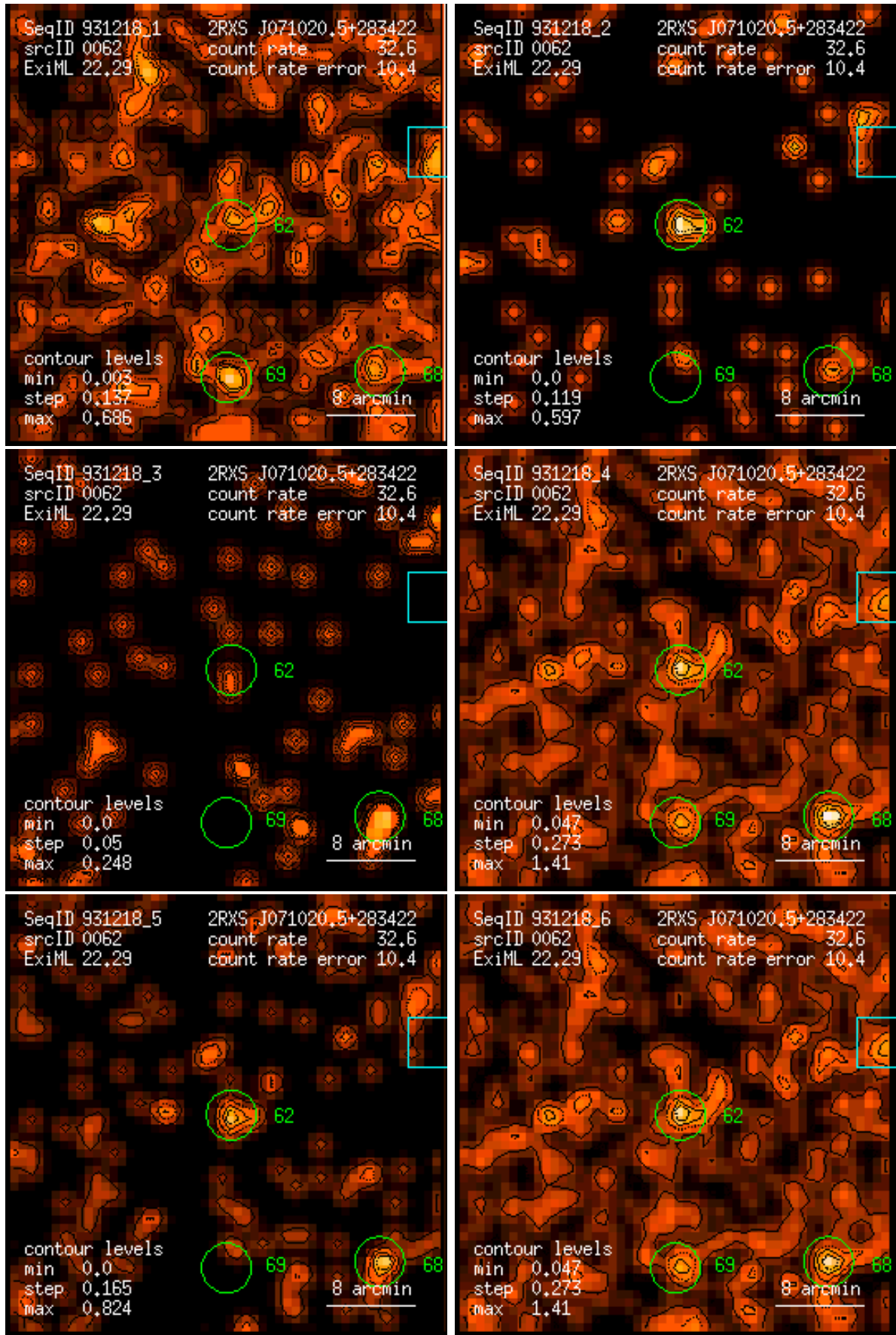
Figure 62: RASS 931218: detection 0062: band rate images, Gaussian filter: (1) PSPC channels 11 – 41, (2) 52 – 90, (3) 91 – 201, (4) 11 – 235, (5) 52 – 201, (6) 11 – 201. Broad band rates in counts/ks. Band rate contour levels in counts/ks/arcmin 2 .
