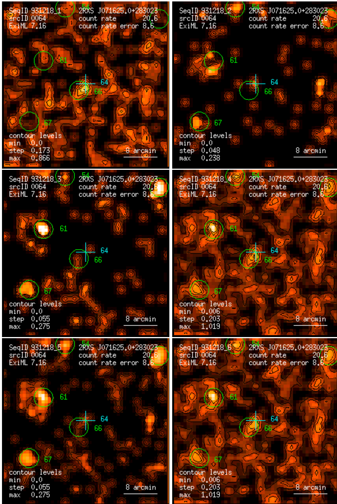
Figure 64: RASS 931218: detection 0064: band rate images, Gaussian filter: (1) PSPC channels 11 – 41, (2) 52 – 90, (3) 91 – 201, (4) 11 – 235, (5) 52 – 201, (6) 11 – 201. Broad band rates in counts/ks. Band rate contour levels in counts/ks/arcmin 2 .
