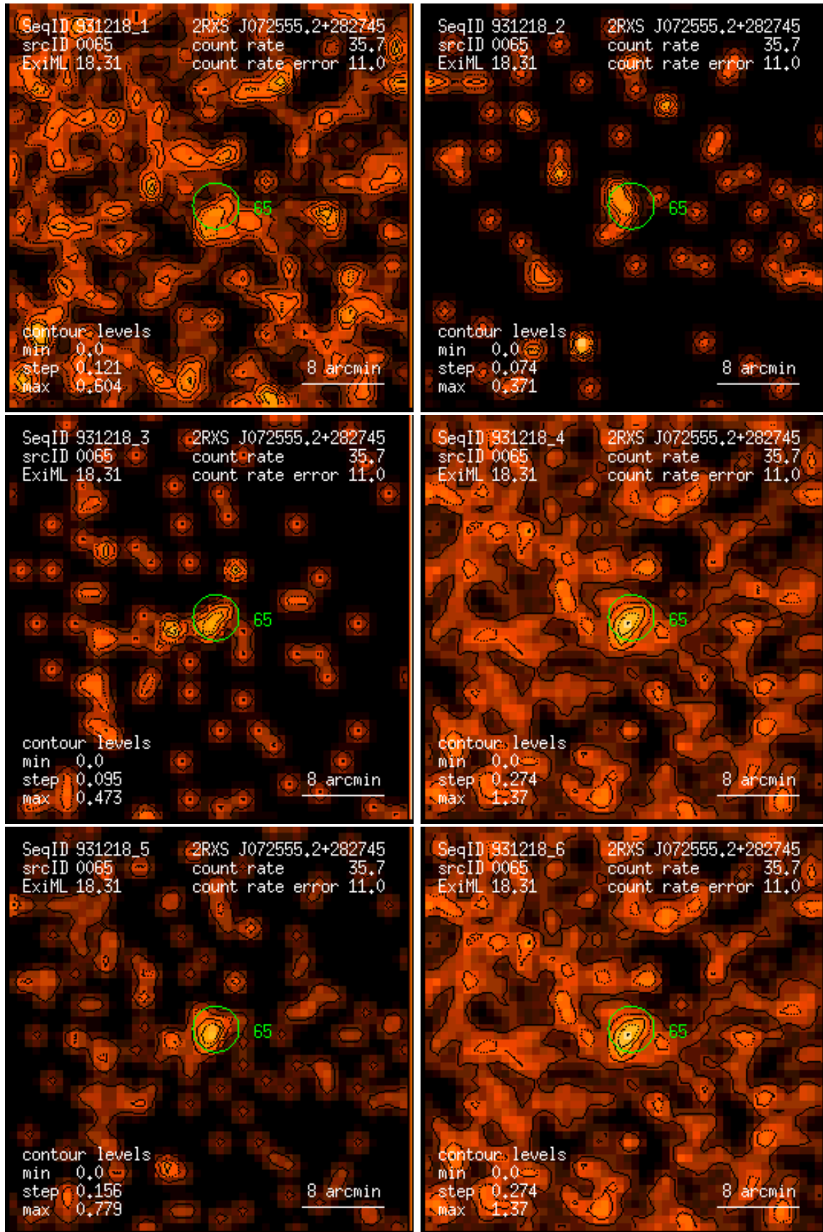
Figure 65: RASS 931218: detection 0065: band rate images, Gaussian filter: (1) PSPC channels 11 – 41, (2) 52 – 90, (3) 91 – 201, (4) 11 – 235, (5) 52 – 201, (6) 11 – 201. Broad band rates in counts/ks. Band rate contour levels in counts/ks/arcmin 2 .
